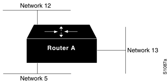
Figure 27 Helper Addresses
