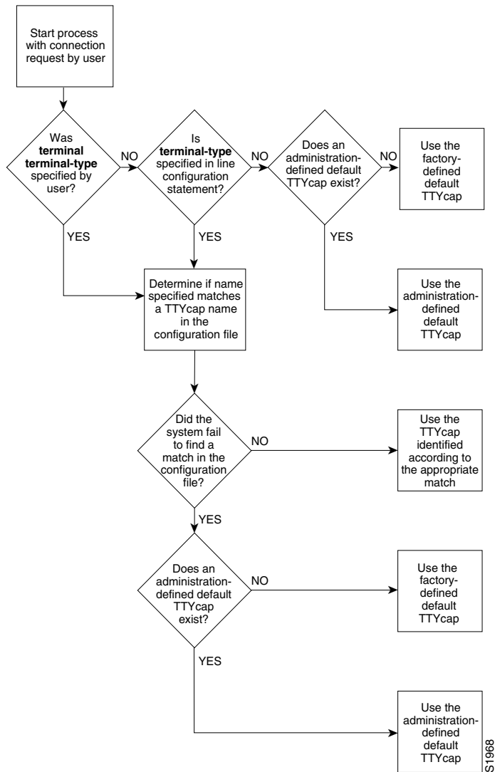
Figure 41 Decision Diagram for Cisco IOS Software Ttycap Selection Process
