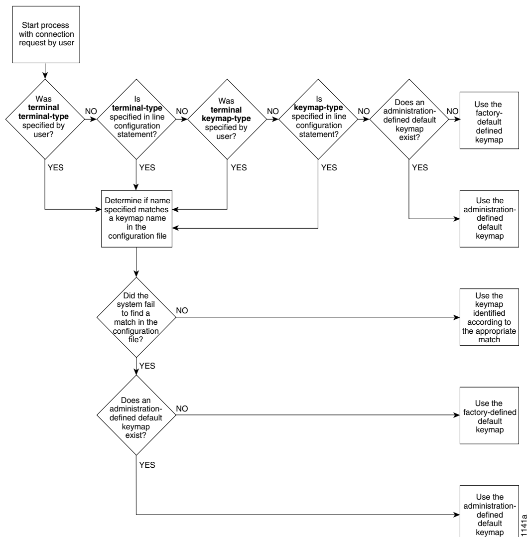
Figure 42 Cisco IOS software Keymap Selection Process
