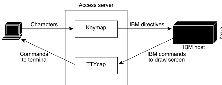
Figure 40 Keymaps and Ttycaps
