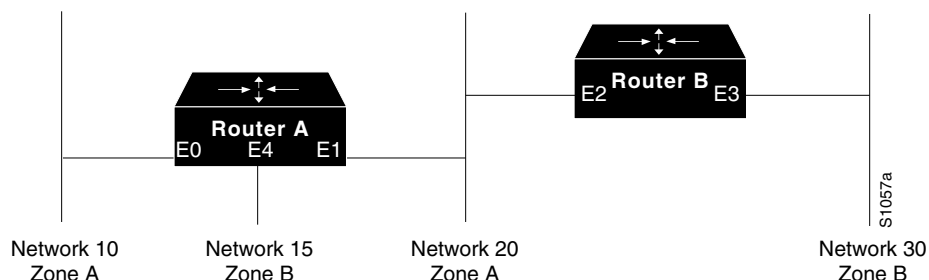
Figure 15-9 Example Topology of Partially Obscured Zone
