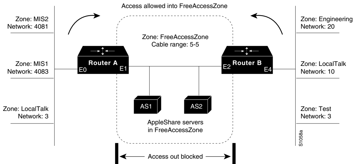
Figure 15-11 Controlling Access to Common AppleTalk Network
