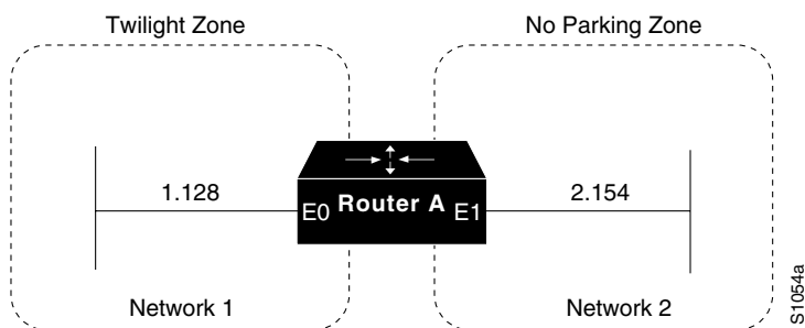
Figure 15-6 Nonextended AppleTalk Routing between Two Ethernet Networks
