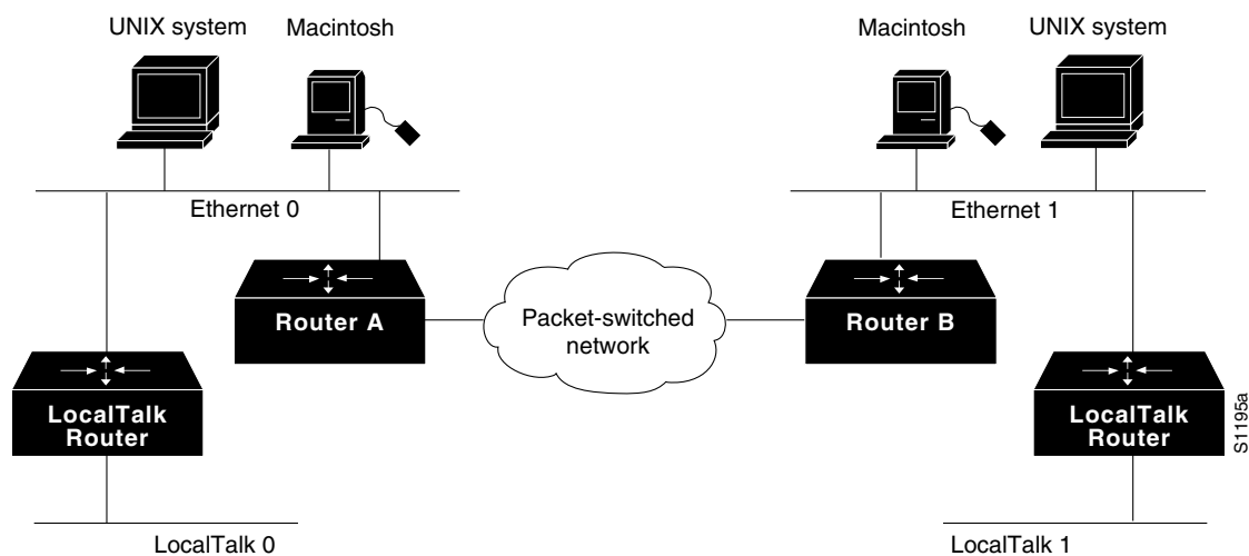
Figure 15-1 IPTalk Configuration Example
