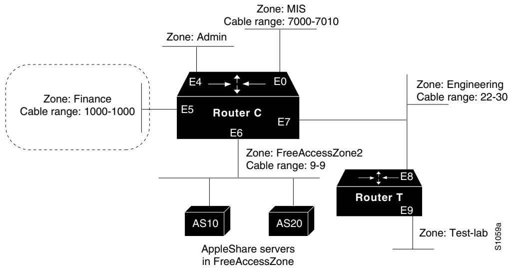
Figure 15-12 Controlling Resource Access among Multiple AppleTalk Zones
