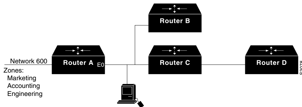
Figure 15-10 GZL and ZIP Reply Filters Sample Topology
