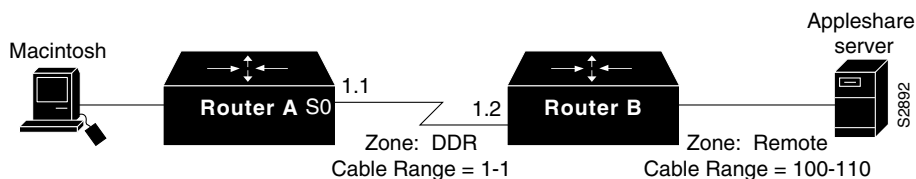
Figure 15-14 AppleTalk over DDR Configuration
