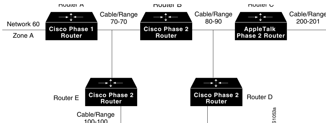
Figure 15-13 Example Network Topology
