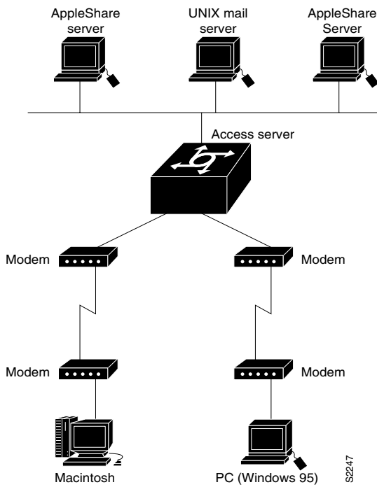
Figure 1-4 Telecommuting Connection
