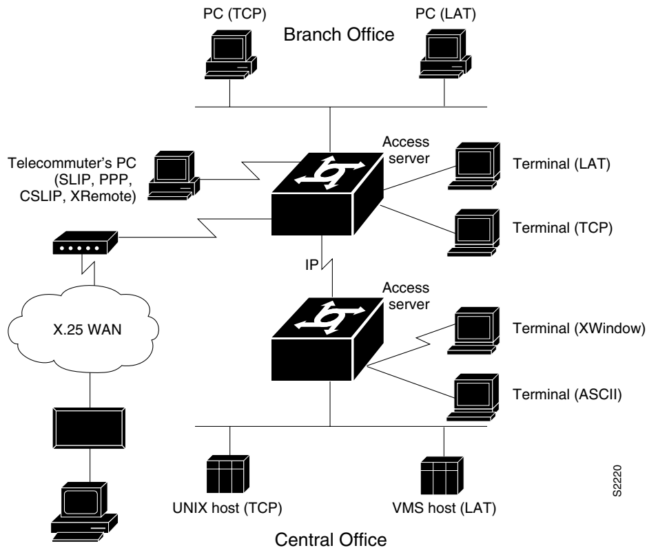
Figure 1-1 Functions of the Access Server
