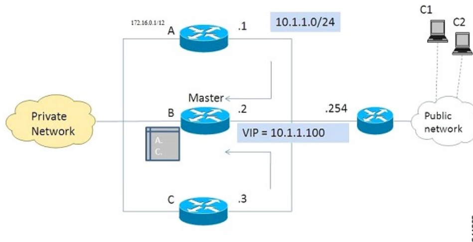
Figure 5: IKEv2 Cluster Load Balancing Solution
