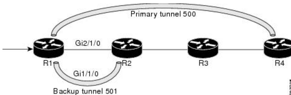
Figure 1: Protected LSPs
