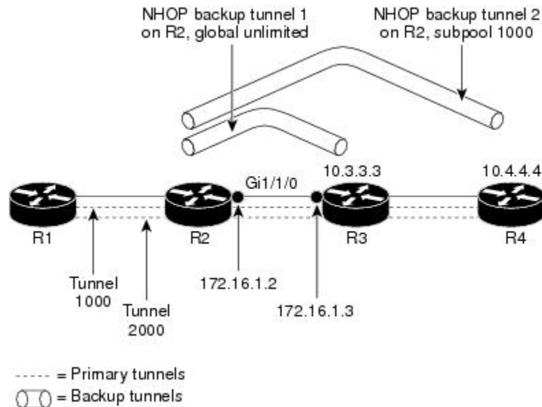
Figure 2: Backup Tunnels
