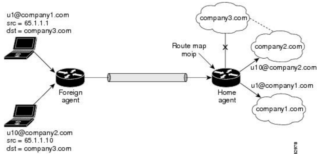
Figure 1: Sample Topology for Mobile IP Home Agent Policy Routing
