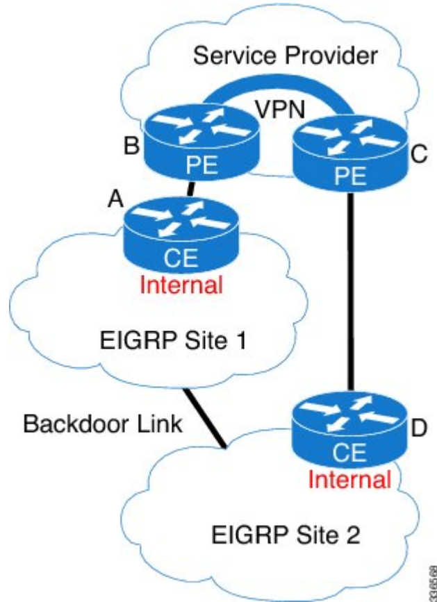
Figure 9: EIGRP 6PE/6VPE Functionality
