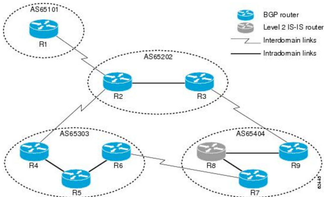
Figure 1: Components in a Generic BGP CLNS Network
