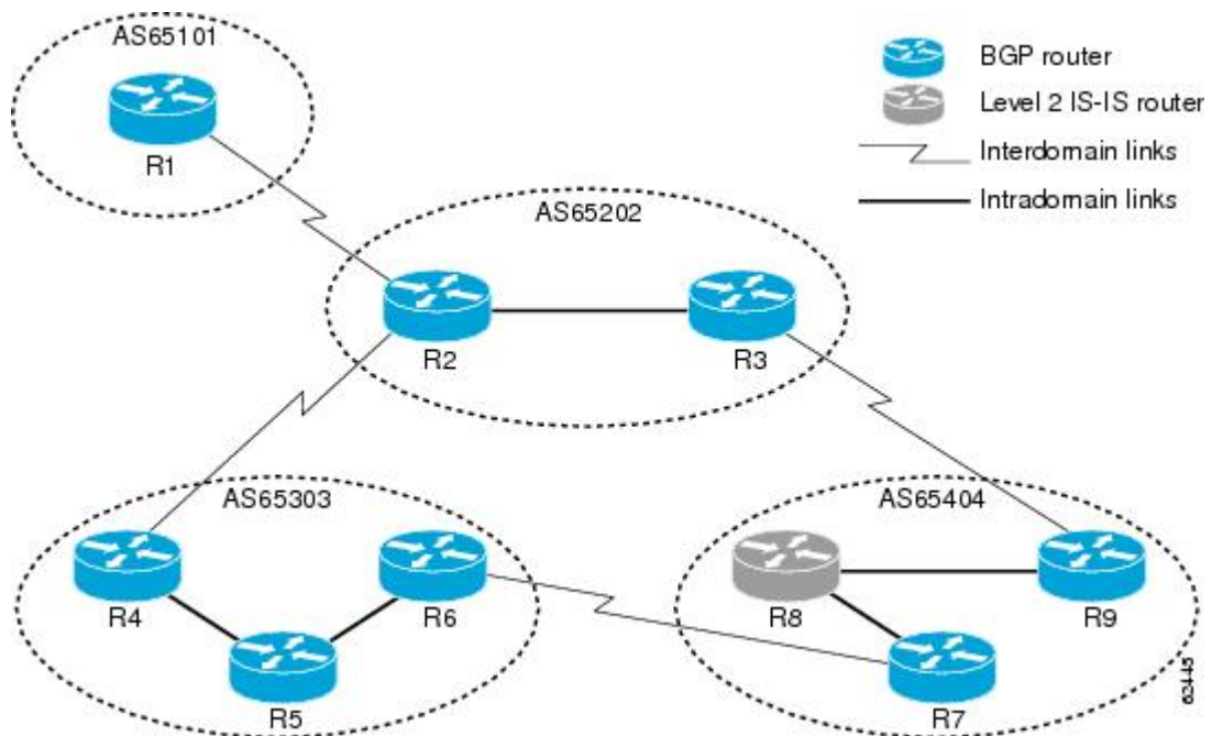
Figure 3: Components in a Generic BGP CLNS Network
