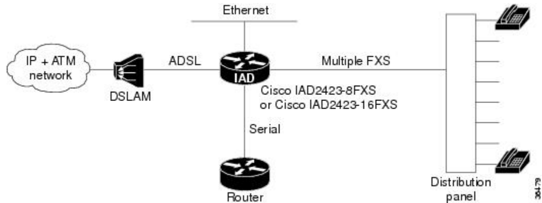
Figure 2: ADSL WAN Interface with T1 Interface to a PBX
