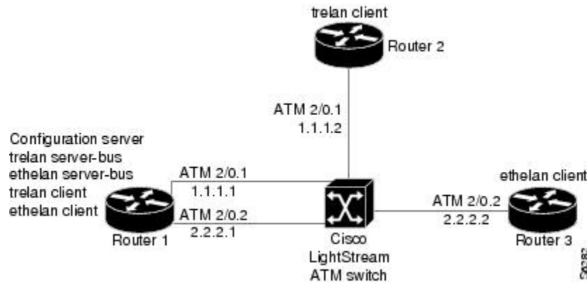
Figure 5 Routing Between Token Ring and Ethernet Emulated LANs
