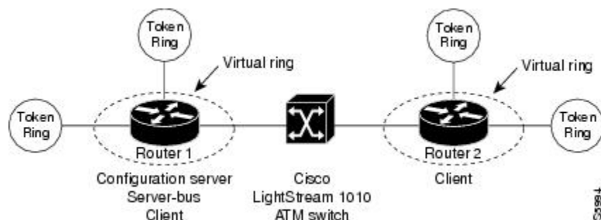
Figure 4 Multiport SRB Token Ring ELAN
