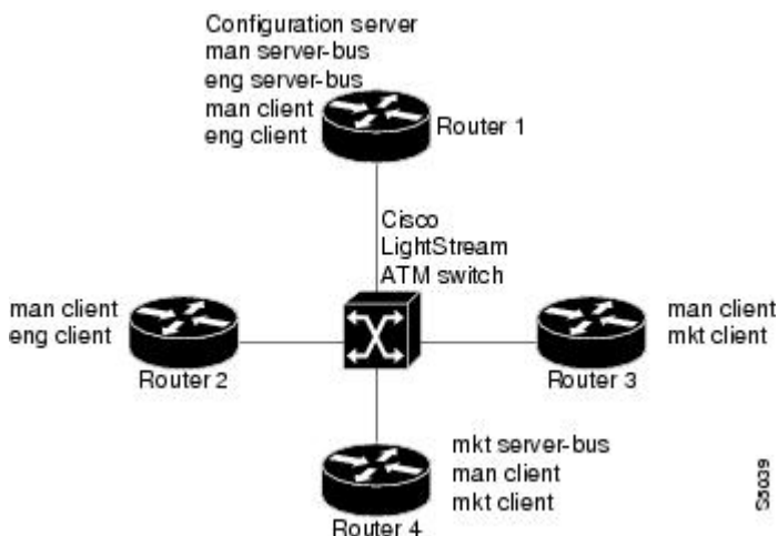
Figure 1 Multiple Emulated LANs
