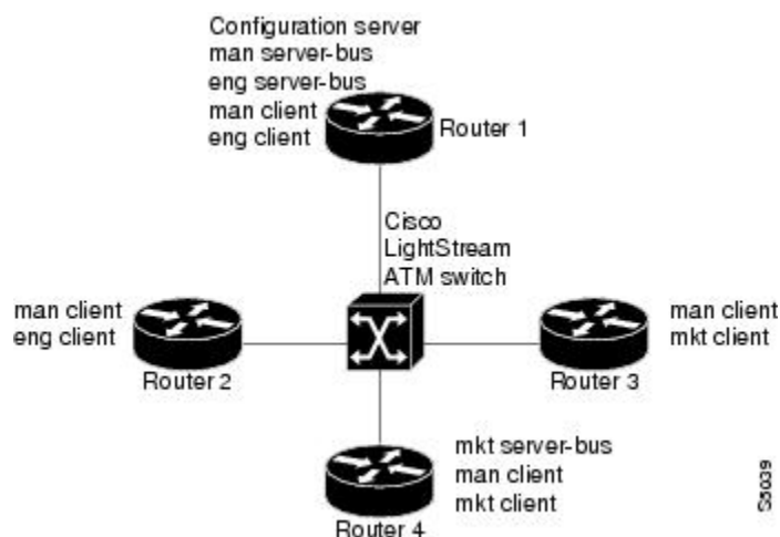
Figure 2 Multiple Emulated LANs with Restricted Membership
