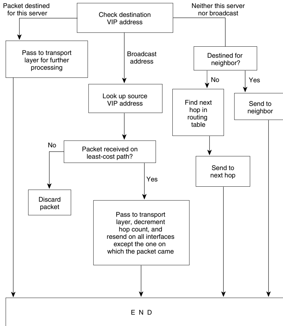
Figure 36-4 The VINES Routing Algorithm Determines the Appropriate Path to a Destination
