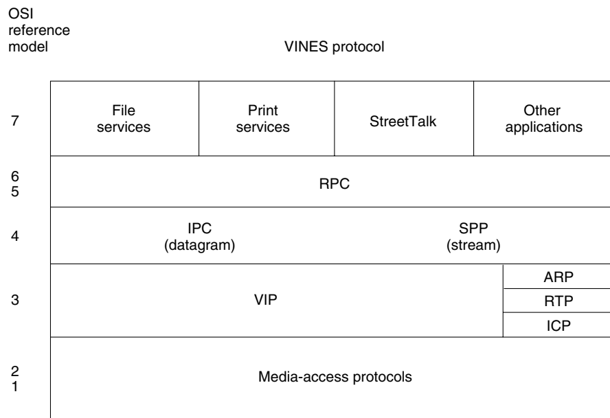
Figure 36-1 The VINES Protocol Stack Consists of Five Separate Levels
