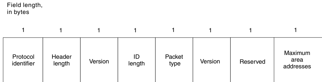
Figure 45-4 IS-IS Packets Consist of Eight Fields
