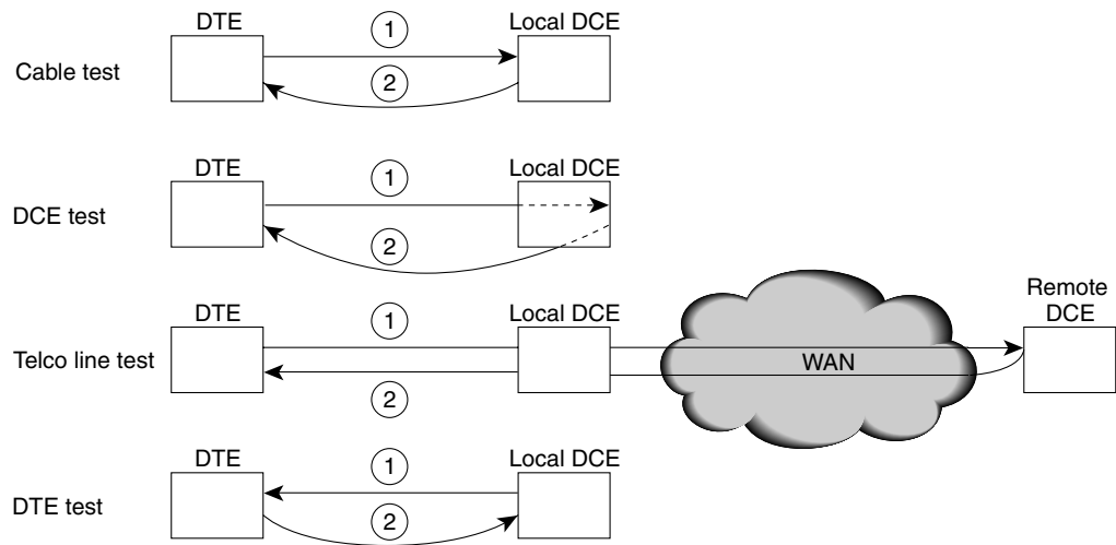
Figure 11-1 HSSI Supports Four Loopback Tests
