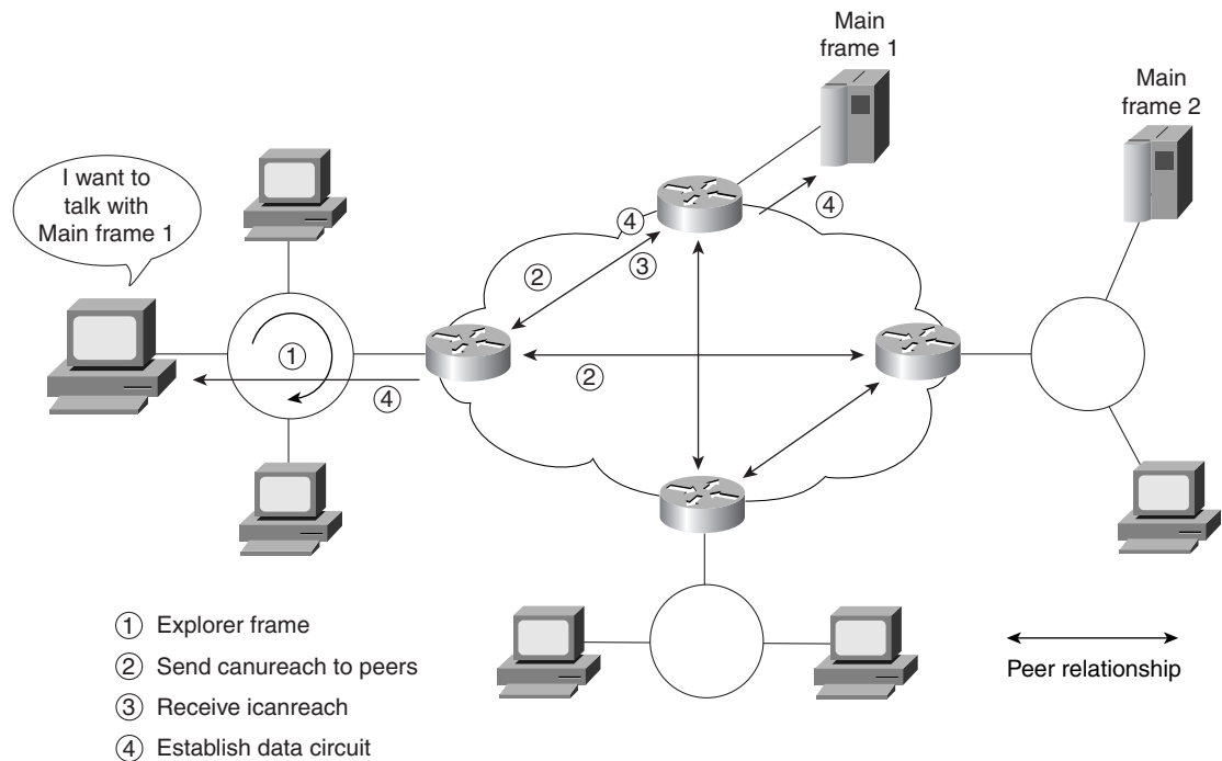
Figure 29-6 DLSw Circuit Establishment Flow
