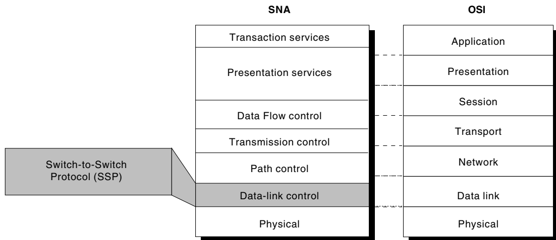
Figure 29-5 SSP Maps to the Data Link Components of SNA and the OSI Reference Model
