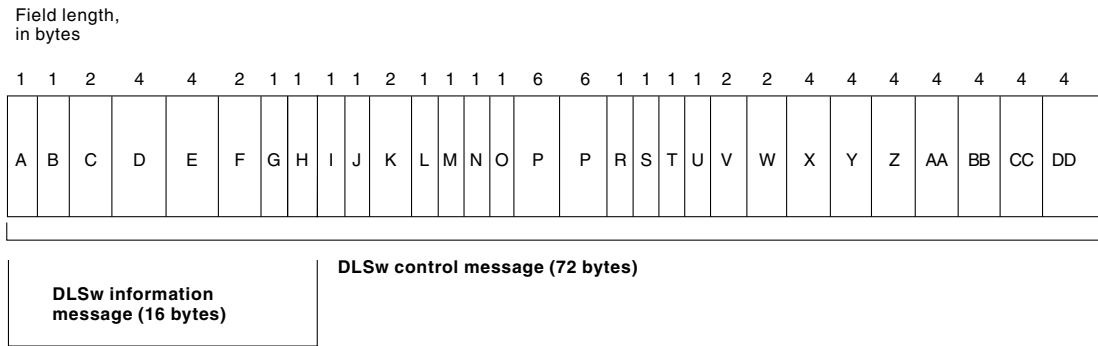
Figure 29-7 DLSw Control and Information Frames Have Their First 16 Bytes in Common
