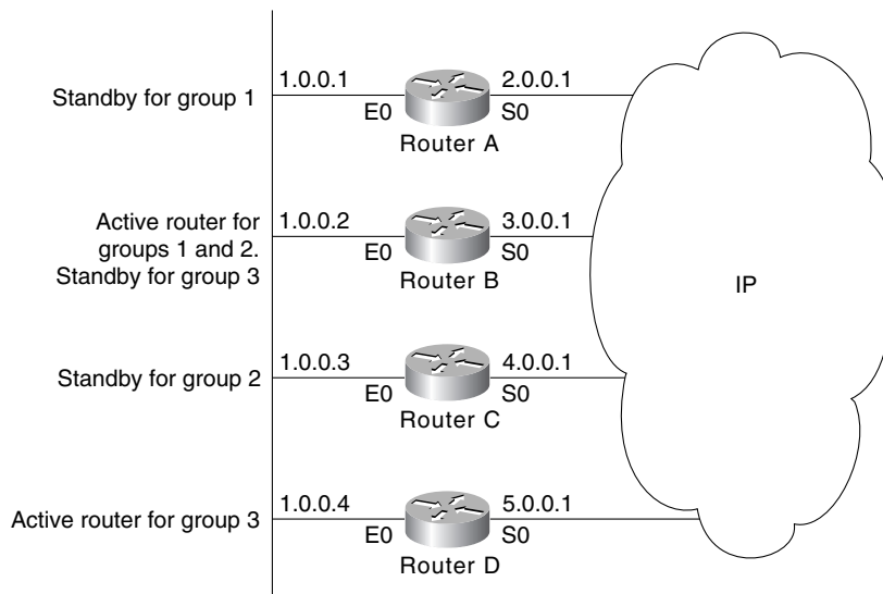
Figure 22-4 Example of hot standby groups.
