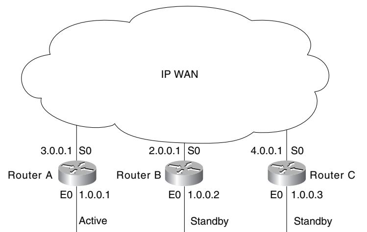
Figure 22-5 A network with tracking configured.
