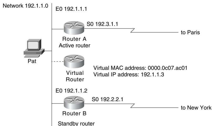
Figure 22-2 HSRP addressing on the Tokyo segment.
