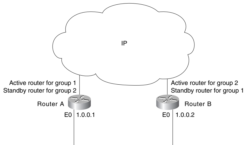
Figure 22-6 Load sharing example.
