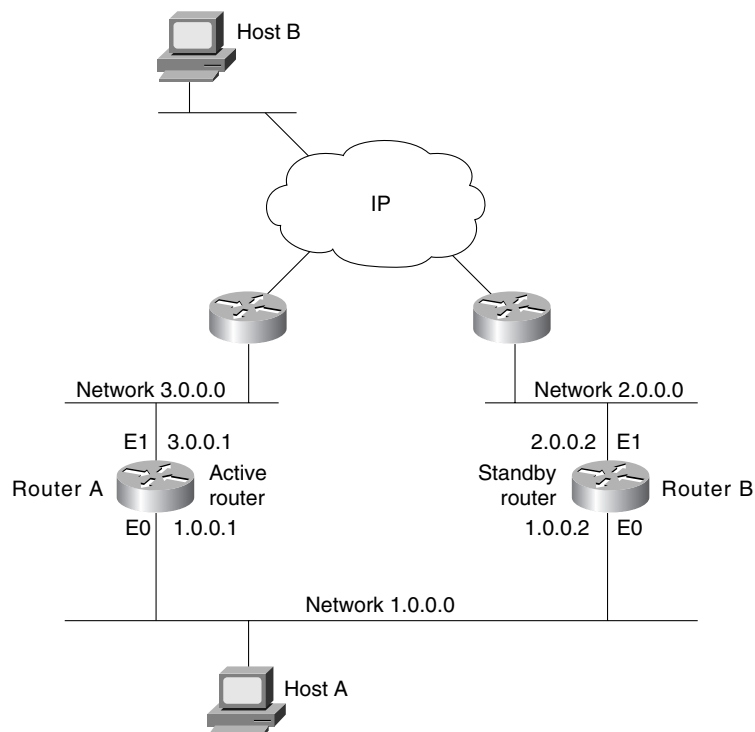
Figure 22-3 Example of a network configured for HSRP.
