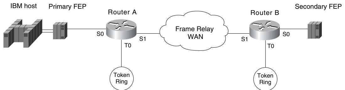
Figure 20-6 Topology for basic STUN: example 2.
