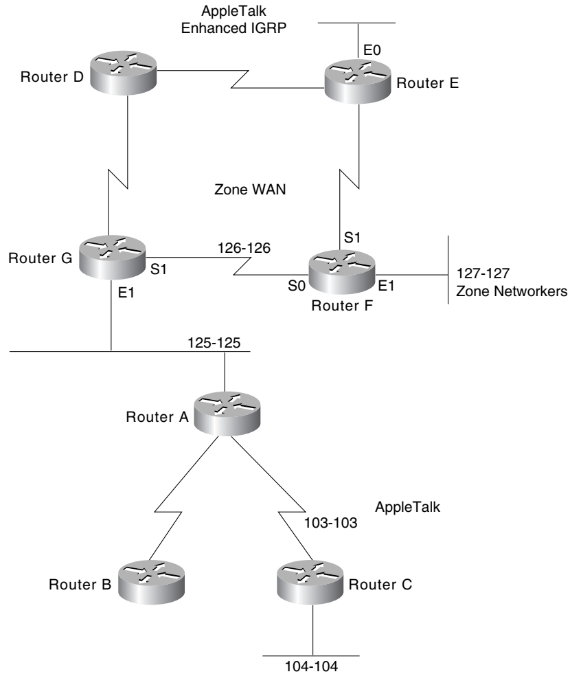
Figure 17-12 Example of adding Enhanced IGRP to an AppleTalk network.
