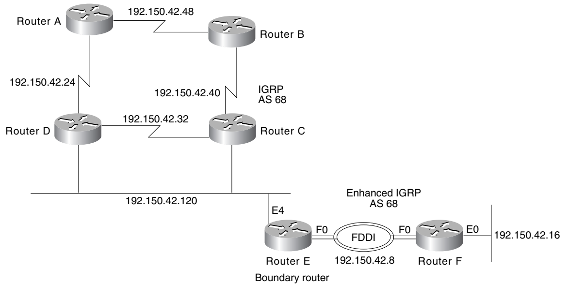
Figure 17-2 Adding Enhanced IGRP to a single IGRP network.
