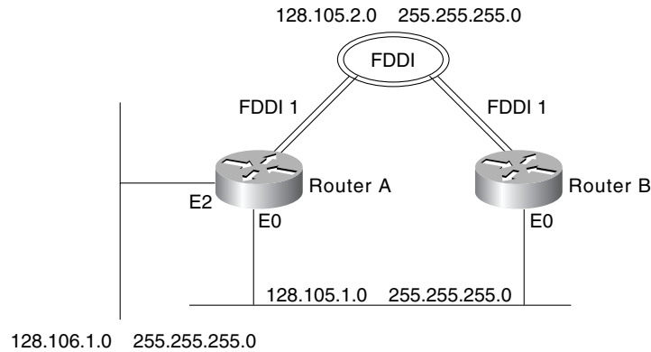
Figure 17-4 Route summarization.
