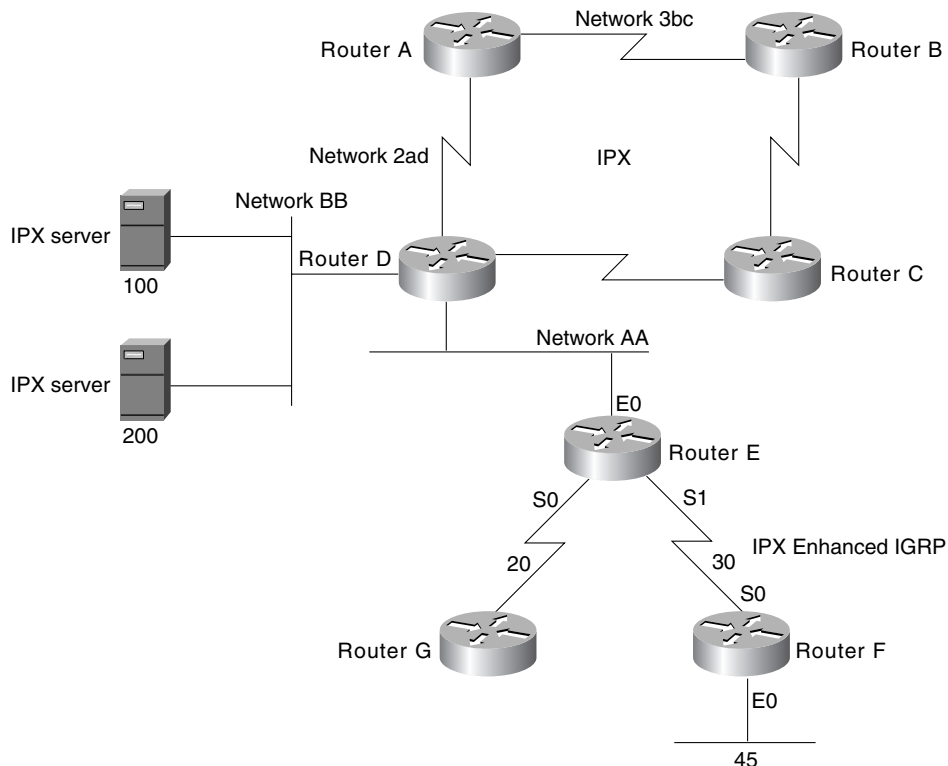
Figure 17-8 Adding Enhanced IGRP to a Novell IPX network.
