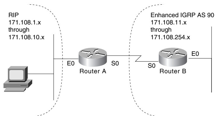
Figure 17-5 Redistributing RIP routes into Enhanced IGRP.
