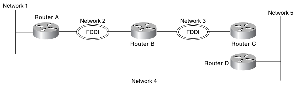
Figure 17-7 Enhanced IGRP Novell IPX optimal path utilization.
