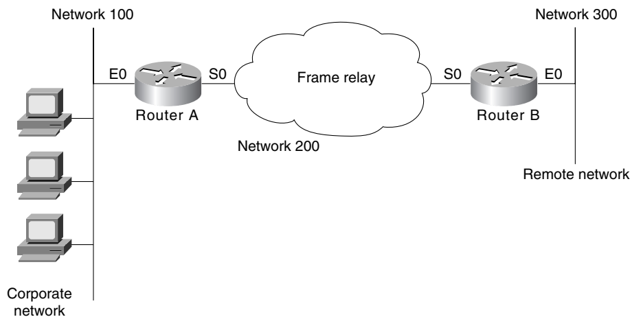
Figure 17-10 Example of incremental SAP updates.
