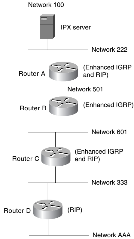
Figure 17-9 IPX metric handling example.
