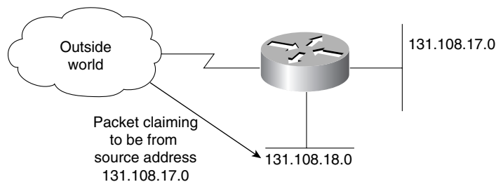
Figure 16-3 A host that is spoofing.
