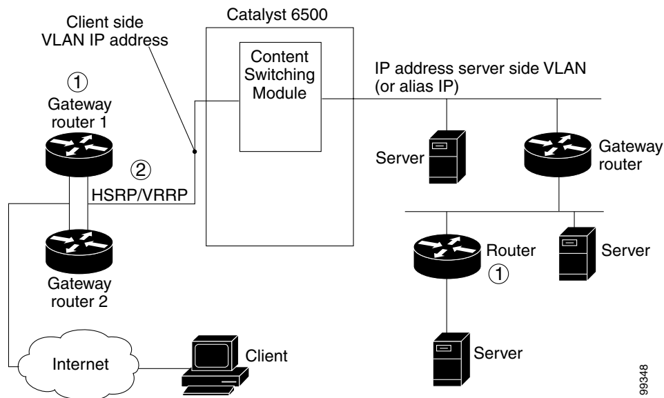
Figure 4-1 Configuring VLANs
