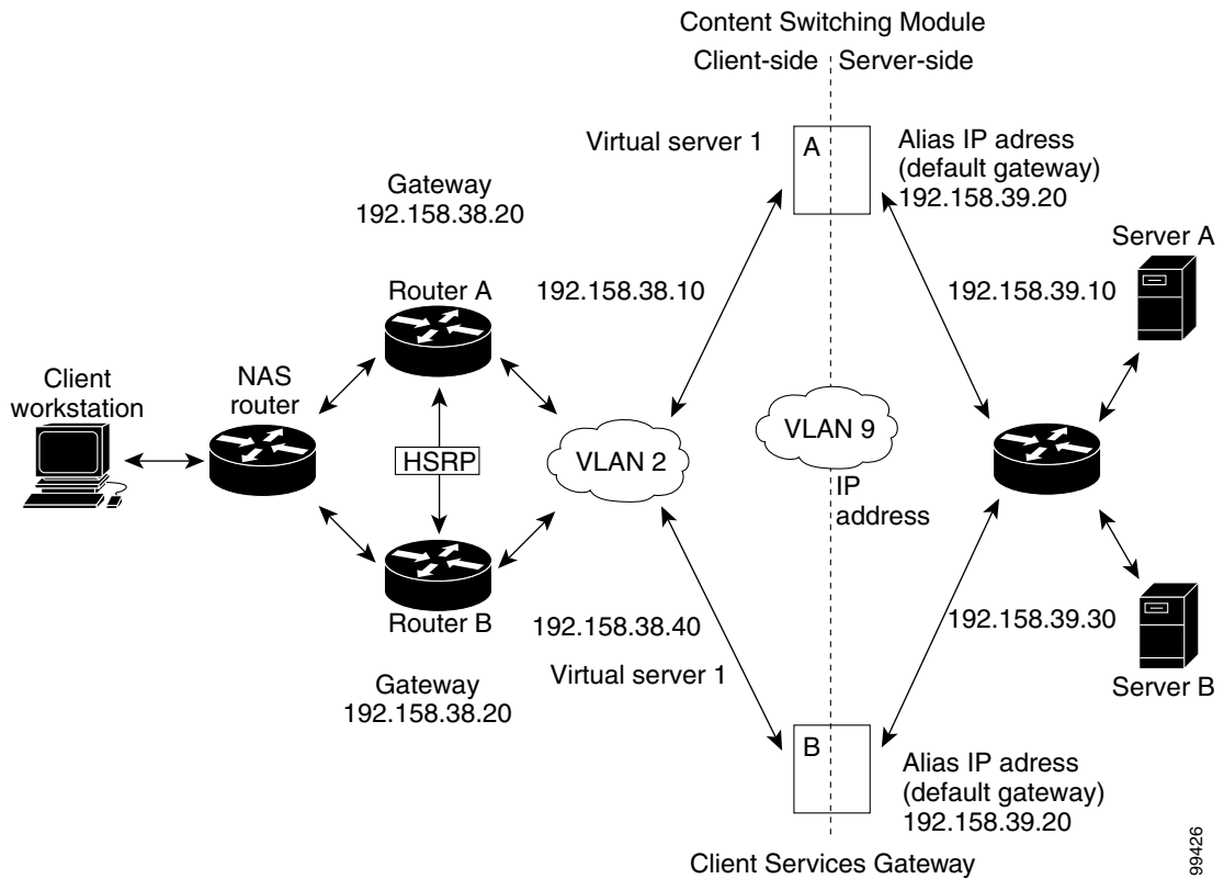
Figure 4-3 Fault-Tolerant Configuration
