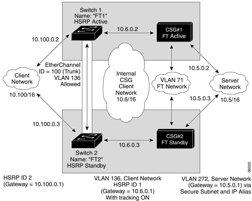
Figure 4-4 HSRP Configuration
