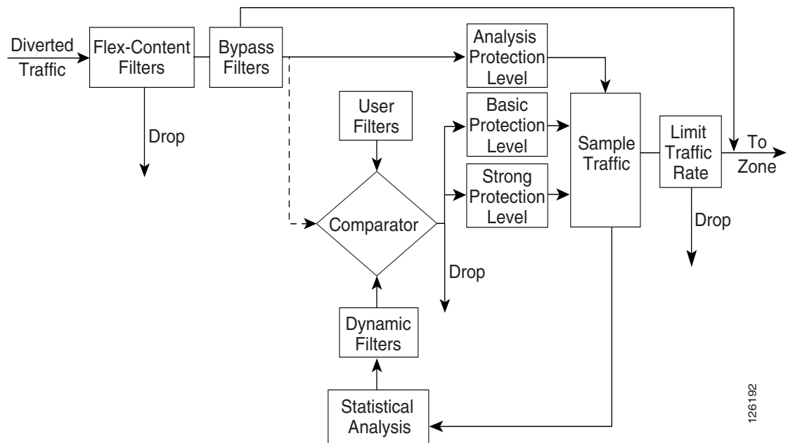
Figure 7-1 Guard Module Filter System
