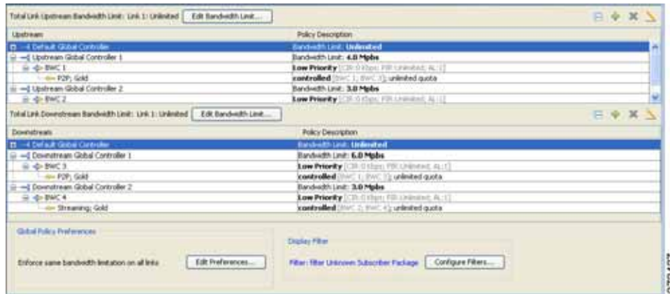
Figure 9-33 Rule Hierarchy
