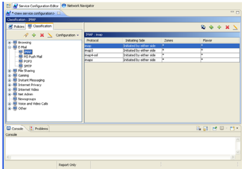
Figure 7-6 Service Elements
