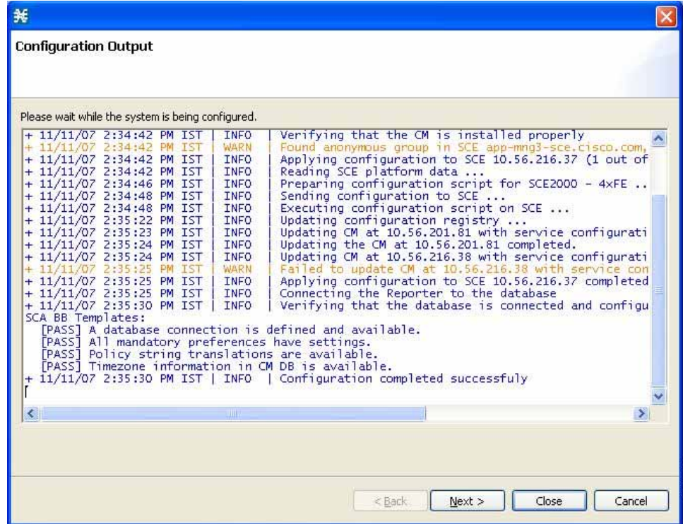
Figure 4-54 Configuration Output
