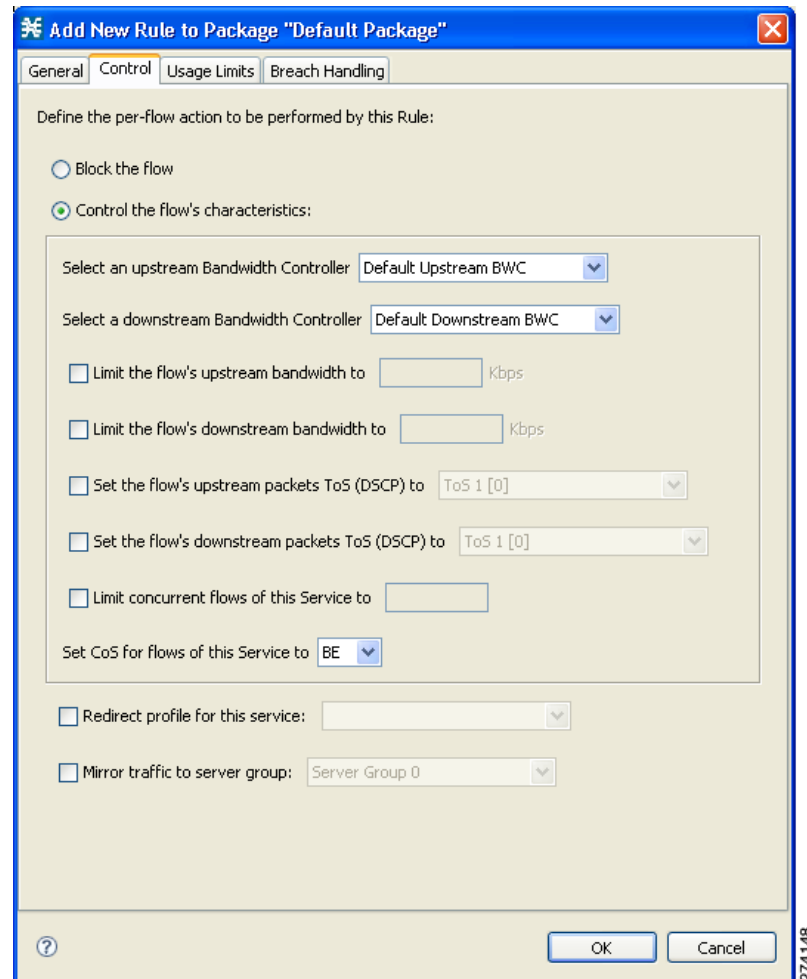
Figure 9-46 Control Tab
