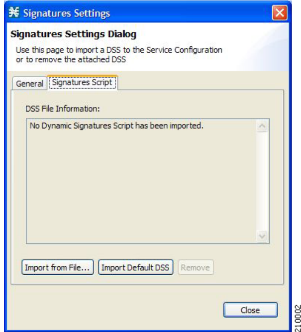
Figure 7-43 Signatures Settings
