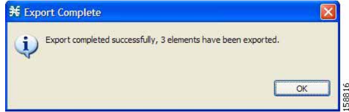
Figure 6-10 Export Complete
