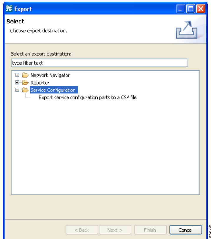
Figure 5-29 Export
