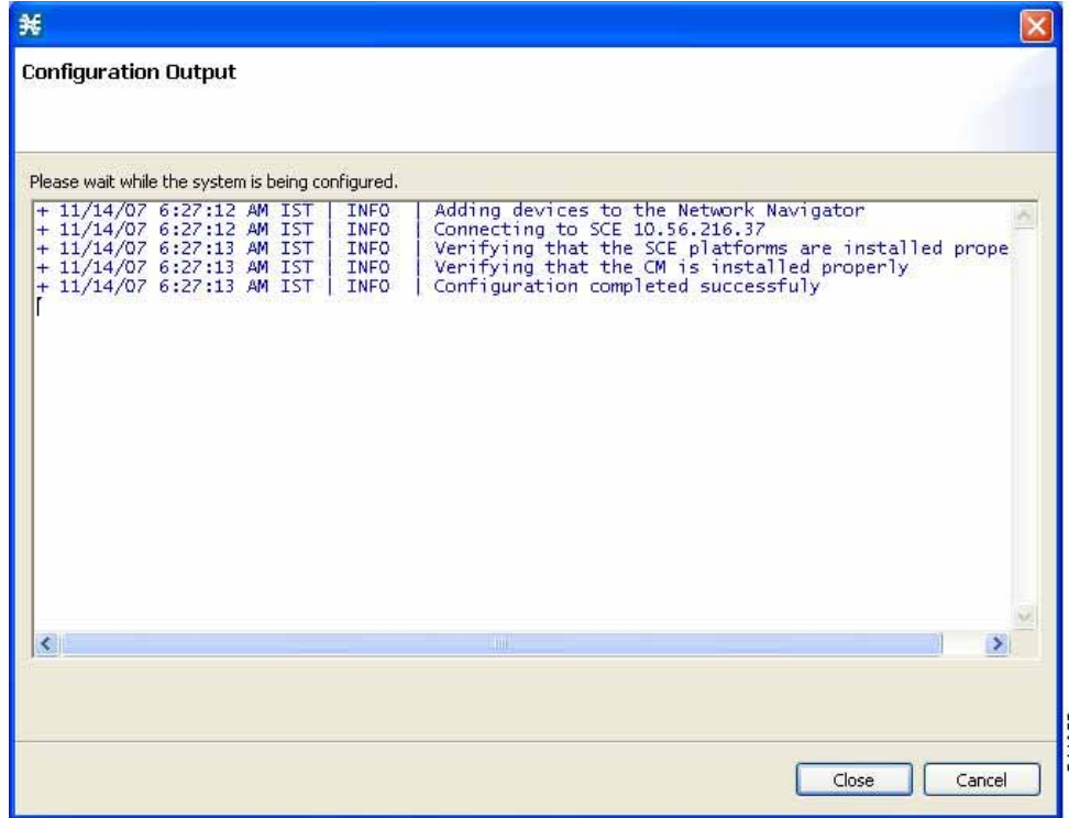
Figure 5-12 Configuration Output
