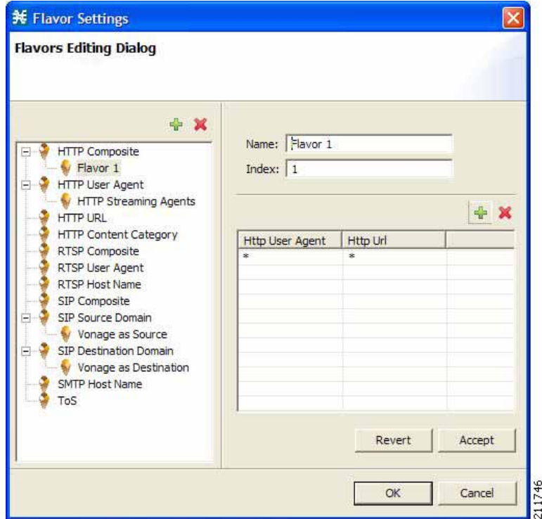
Figure 7-50 Flavor Settings
