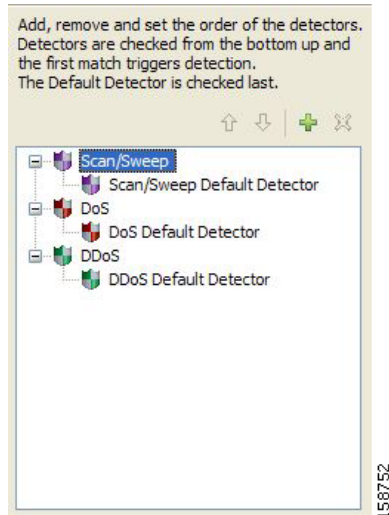
Figure 10-2 Detector Tree
