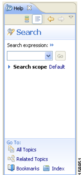
Figure 4-72 Help
