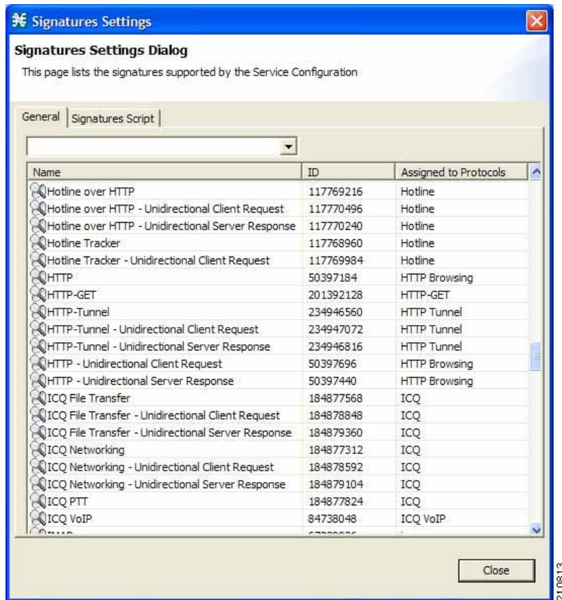
Figure 7-34 Signatures Settings
