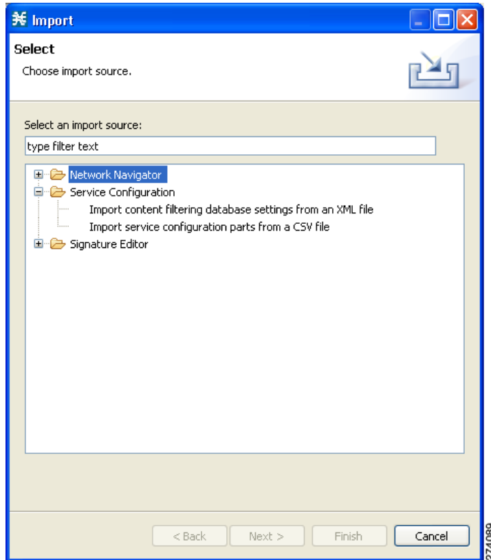
Figure 7-54 Import
