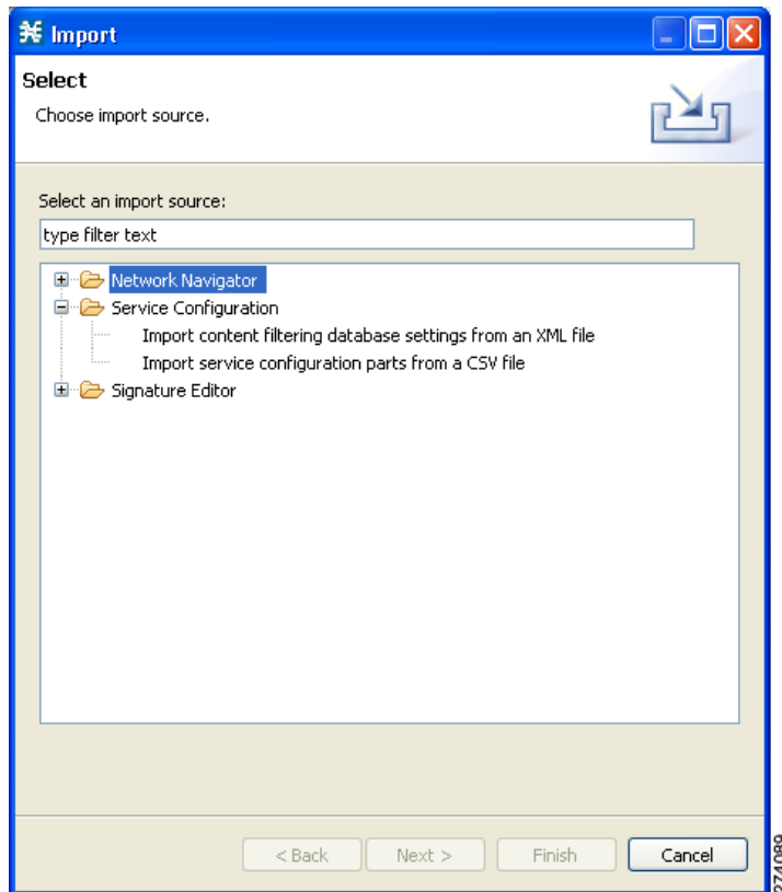
Figure 5-31 Import
