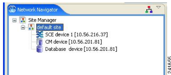
Figure 4-55 Network Navigator
