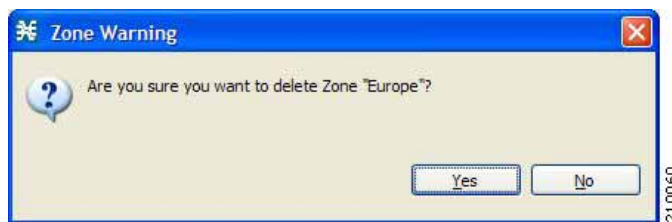
Figure 7-31 Zone Warning
