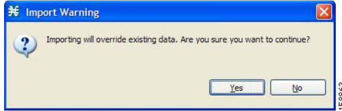
Figure 7-37 Import Warning
