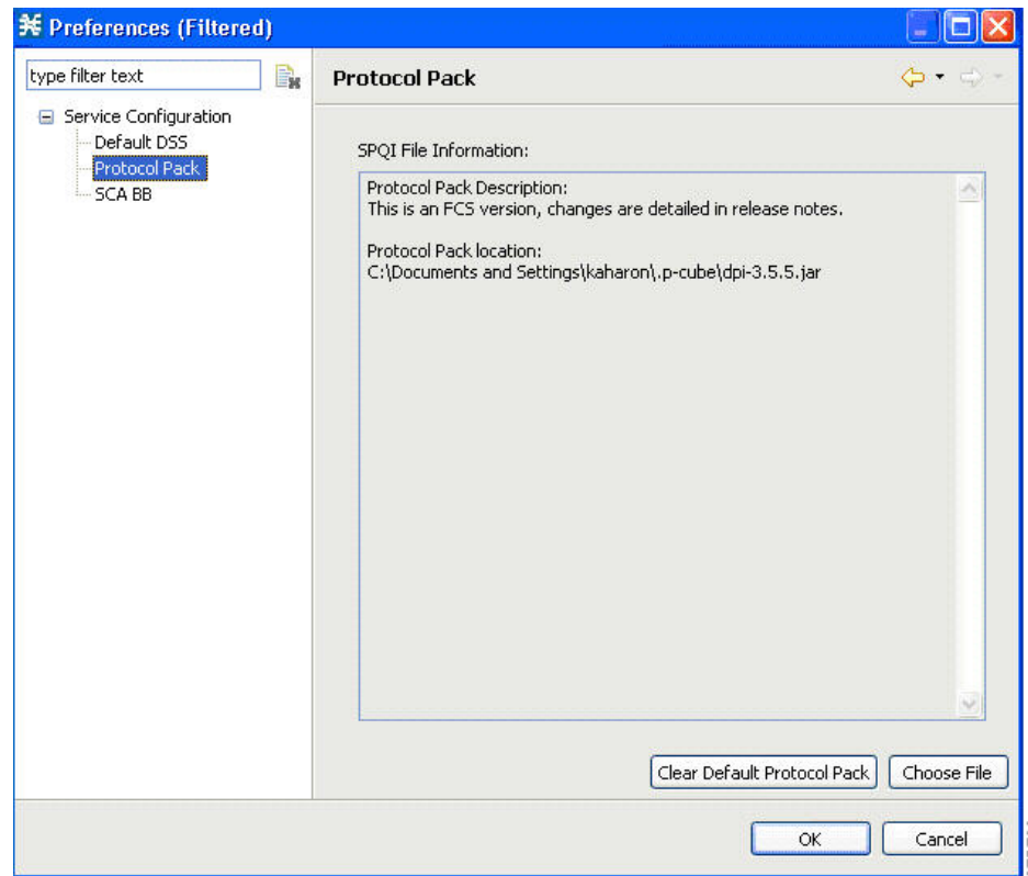
Figure 4-22 Preferences (Filtered)
