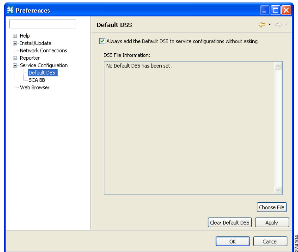
Figure 7-40 Preferences
