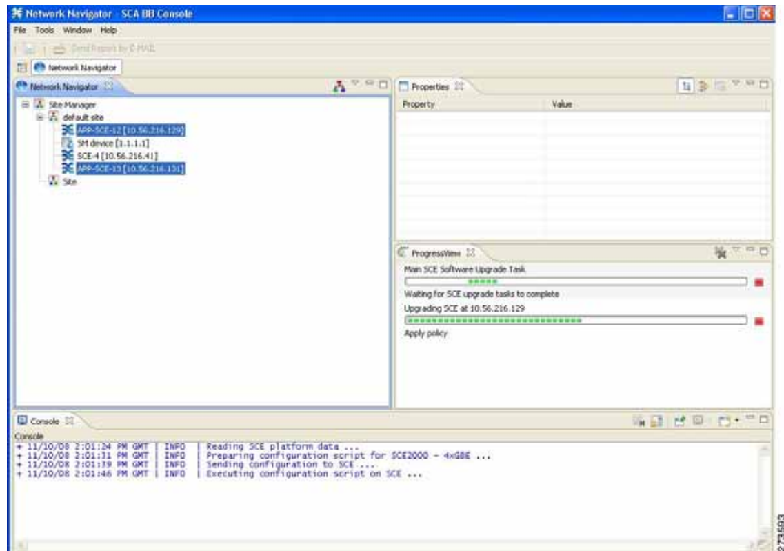
Figure 4-15 Progress
