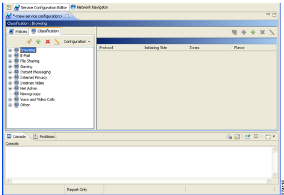
Figure 7-5 Classification Tab
