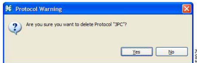
Figure 7-23 Protocol Warning
