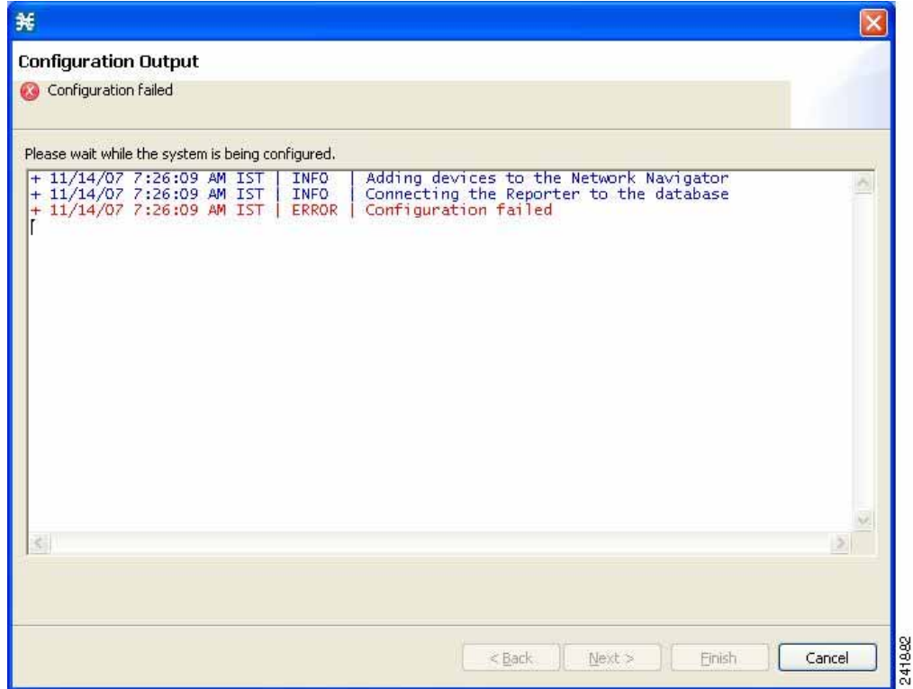
Figure 4-63 Configuration Output
