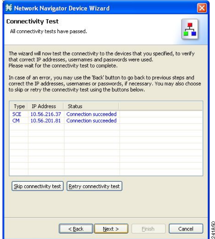
Figure 5-10 Connectivity Test
