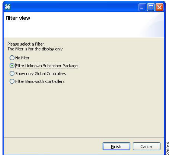
Figure 9-5 Filter View
