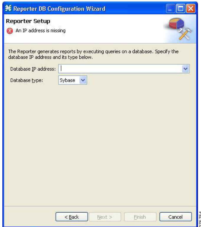
Figure 4-47 Reporter Setup
