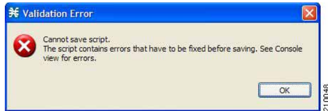
Figure 12-11 Validation Error
