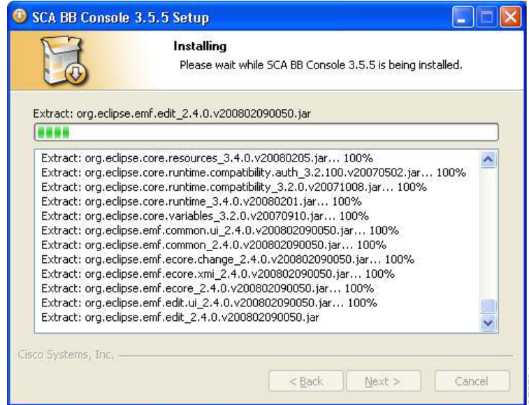
Figure 4-4 Installing
