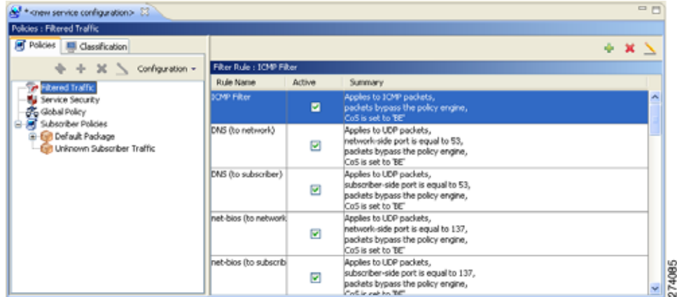
Figure 10-14 Filter Rules
