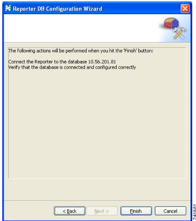
Figure 4-62 Confirmation
