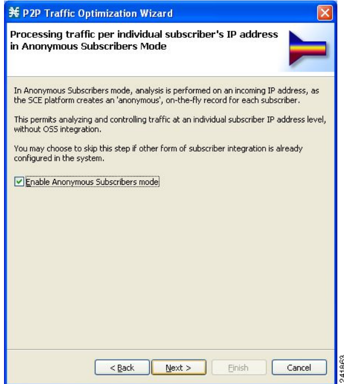
Figure 4-49 Anonymous Subscribers
