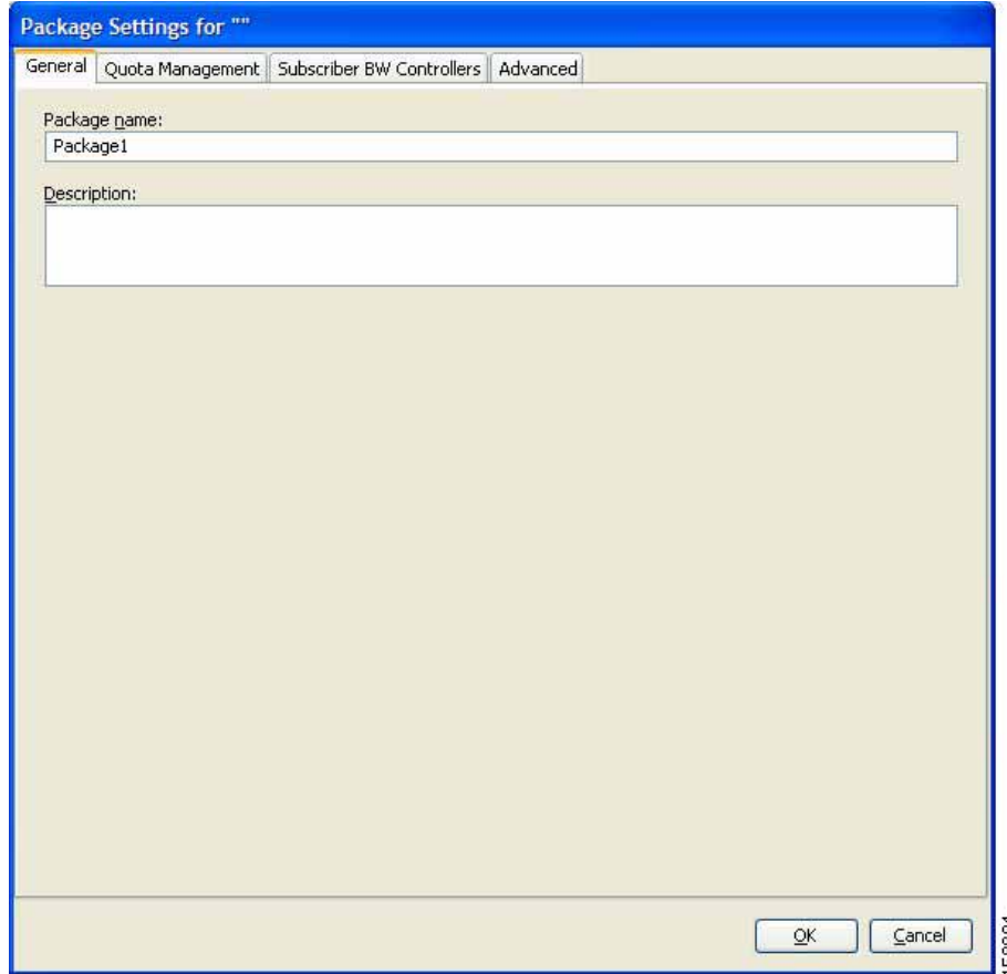
Figure 9-41 Package Settings
