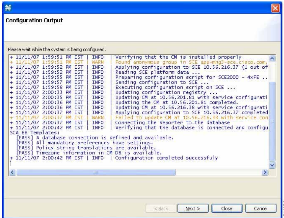
Figure 4-37 Configuration Output
