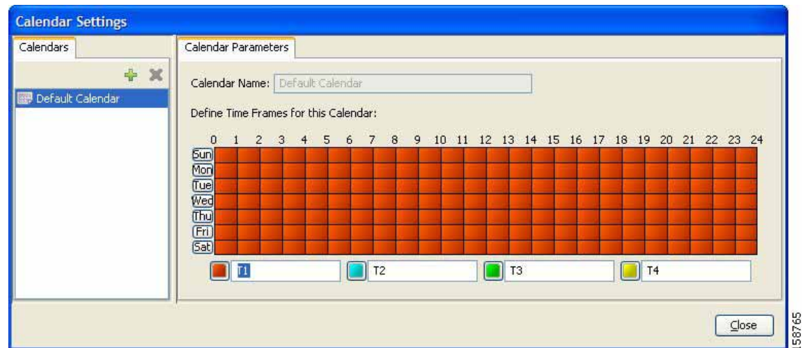
Figure 9-57 Calendar Settings
