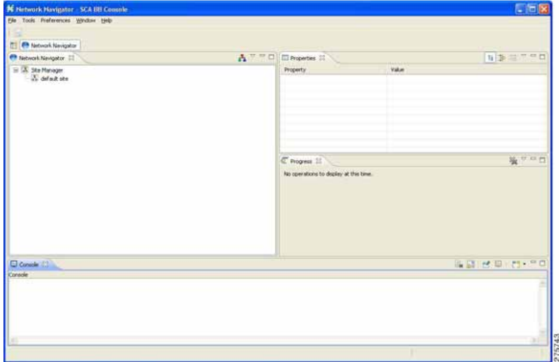
Figure 4-26 Network Navigator
