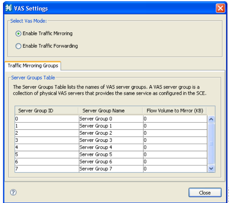
Figure 10-38 Traffic Mirroring Groups Tab
