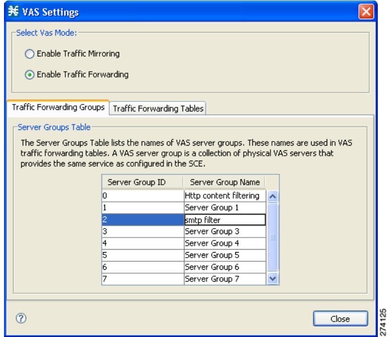
Figure 10-37 Traffic Forwarding Groups Tab
