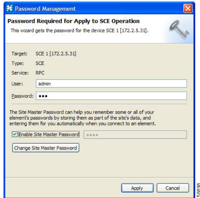
Figure 5-2 The Password Management Dialog Box
