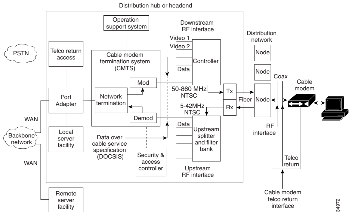
Figure 1-1 DOCSIS Two-Way Architecture
