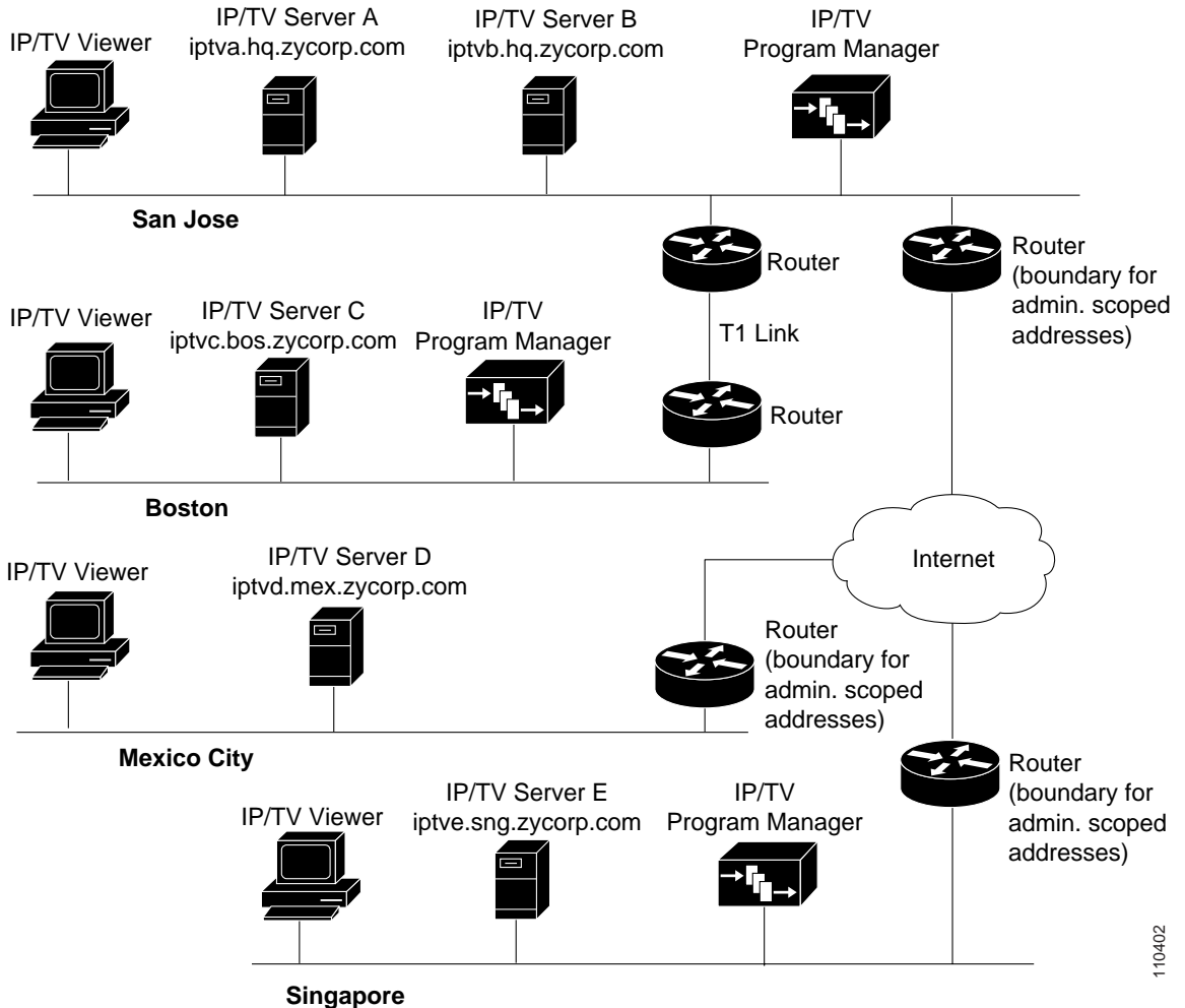
Figure 11-1 Sample Network
