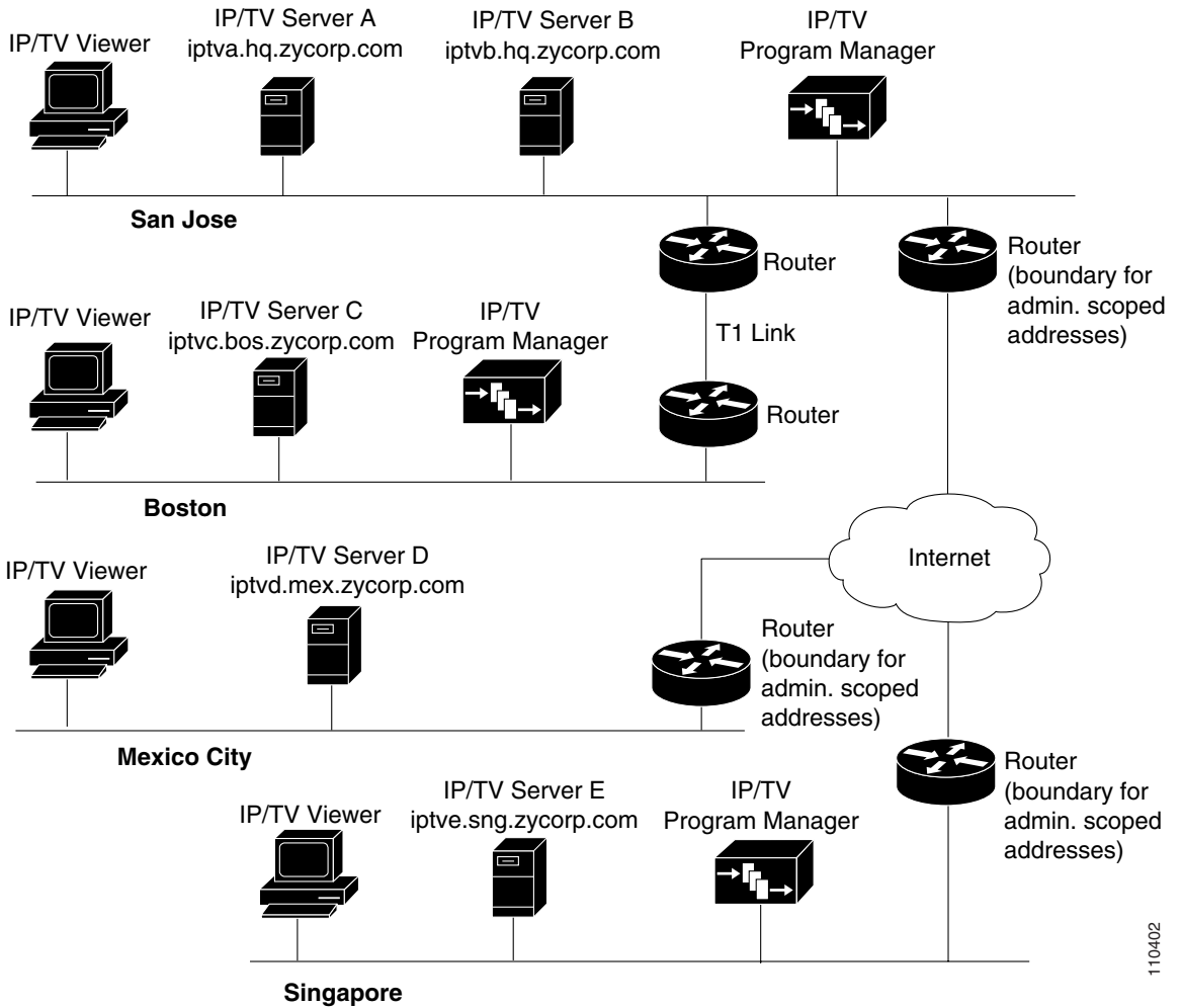
Figure 11-1 Sample Network
