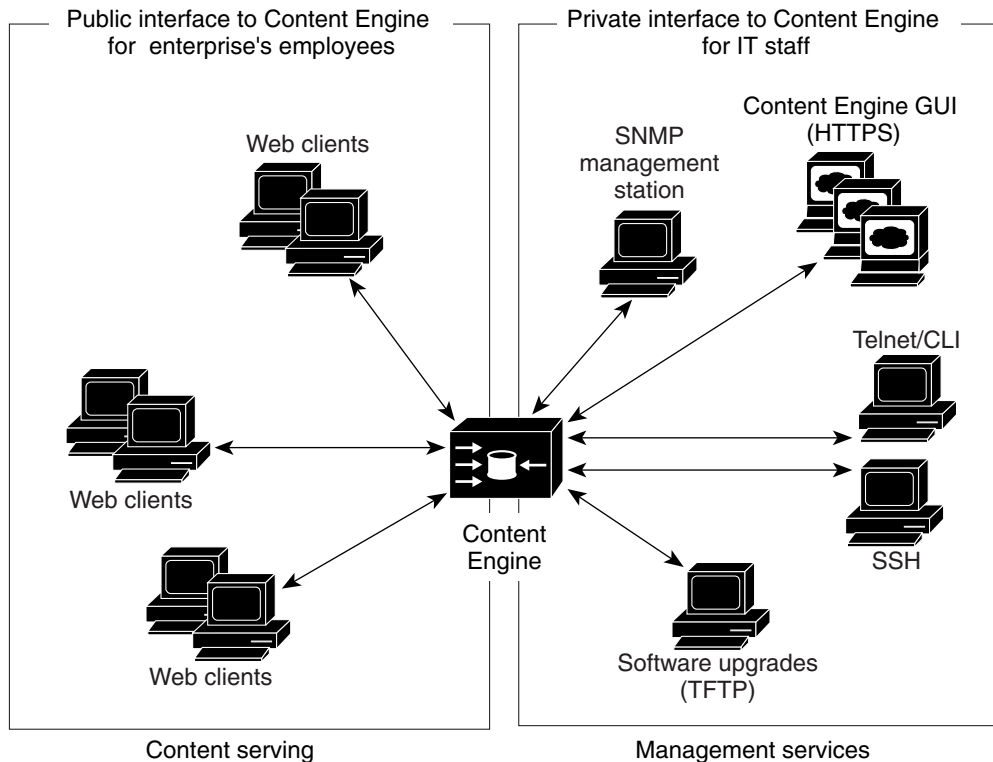
Figure 18-1 Using IP ACLs to Control Access to Specific Interfaces on a Standalone Content Engine
