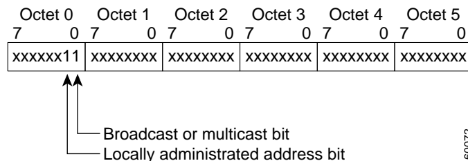
Figure B-1 IEEE 802.3 MAC Address Format
