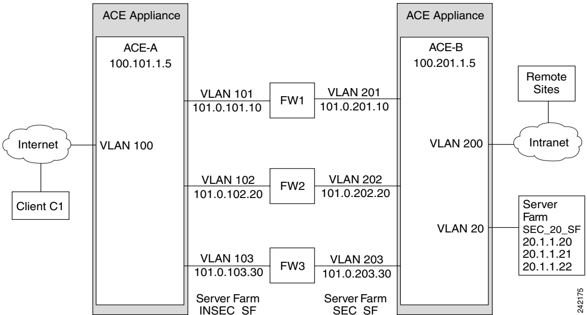
Figure 6-2 Stealth Firewall Configuration (Dual ACEs Only)
