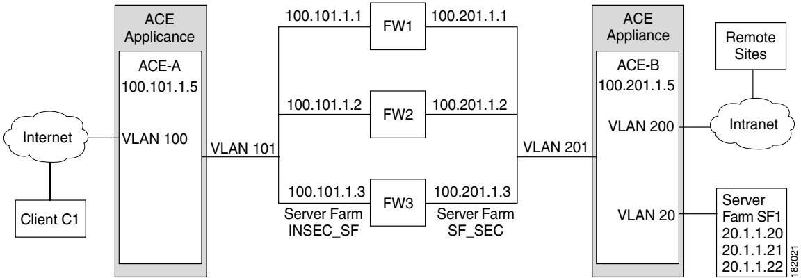
Figure 6-1 Standard Firewall Configuration
