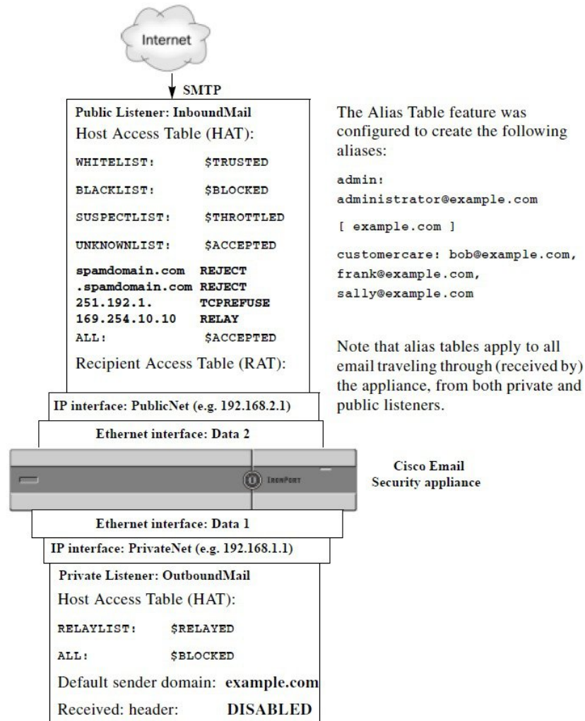
Figure 49: 为邮件网关定义的别名表
