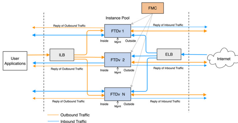
図 36: Secure Firewall Threat Defense Virtual Auto Scale の導入例の図
