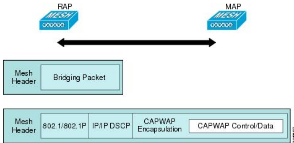
Figure 23: Encapsulating Mesh Traffic
