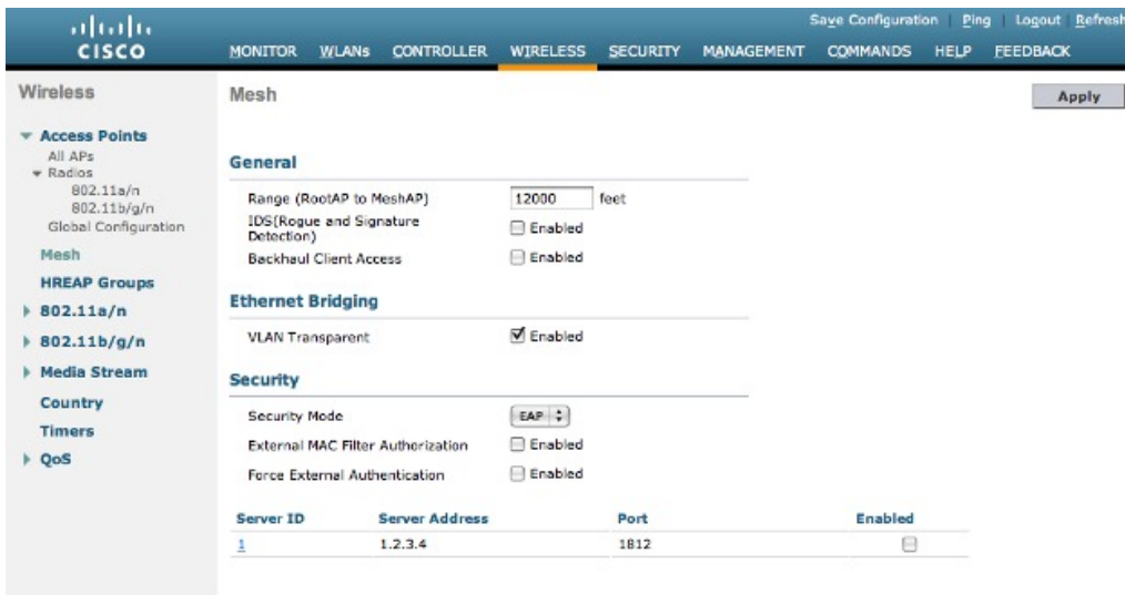
Figure 5: Mesh Page
