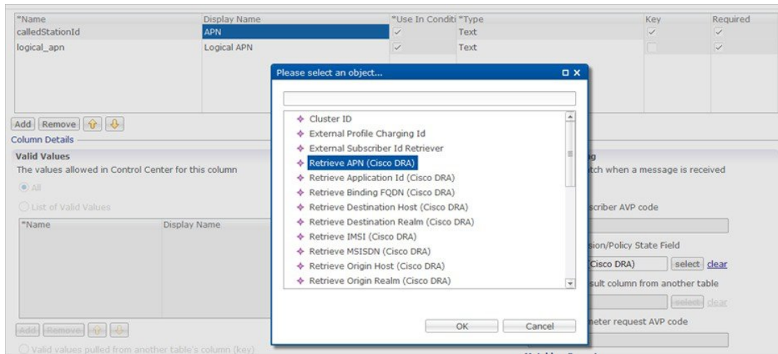
Figure 71: Adding AVPs
