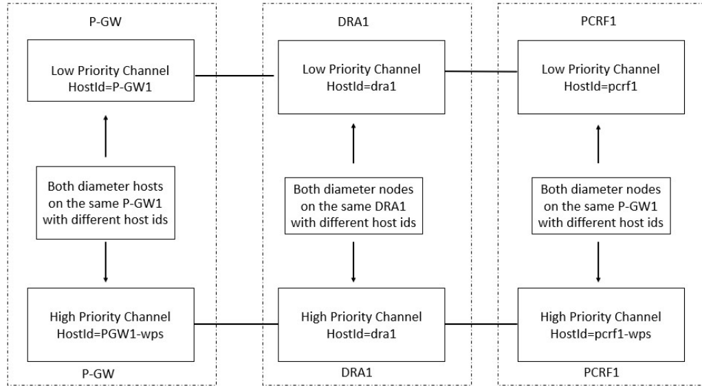
Figure 136: High-Level Overview of Low and High Priority Channels over Rx Interface
