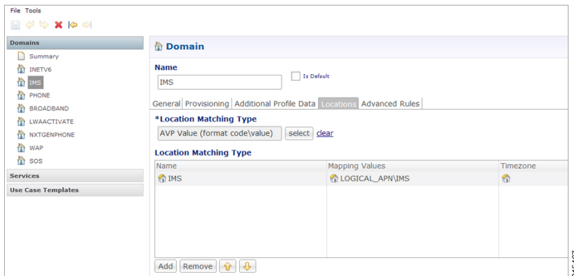
Figure 3: Domain Locations
