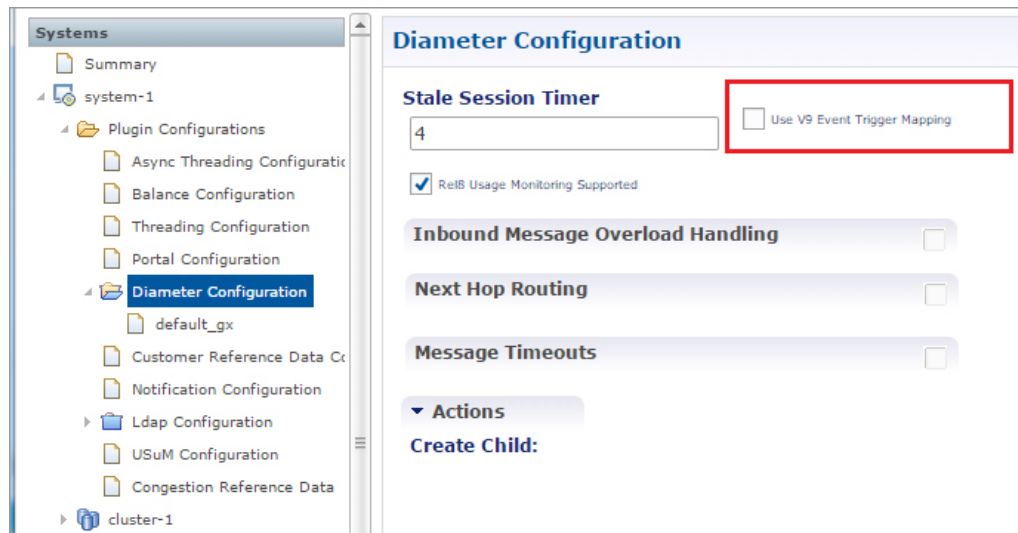
Figure 19: Diameter Configuration
