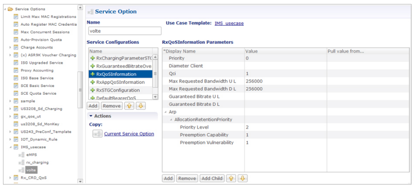
Figure 5: RxQoSInformation Service
