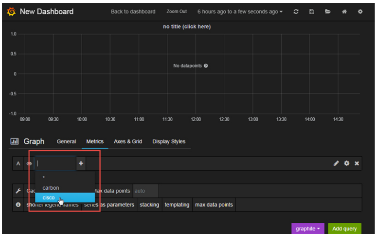
Figure 39: Metric Selection
