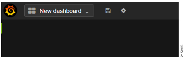
Figure 33: Blank Dashboard
