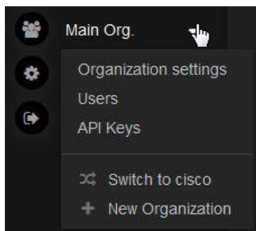
Figure 27: New Organization
