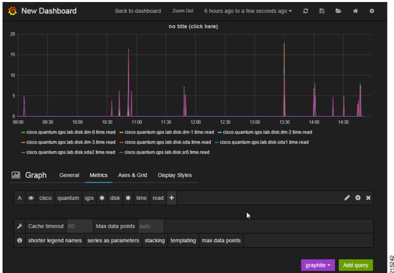
Figure 40: Aggregation Functions
