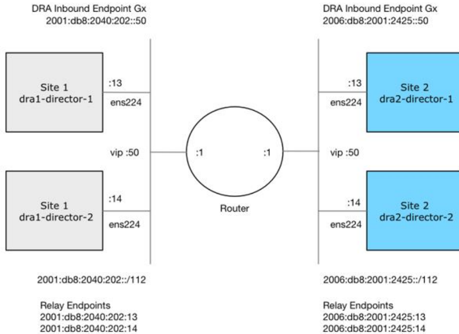
Figure 54: Example of Relay Endpoints
