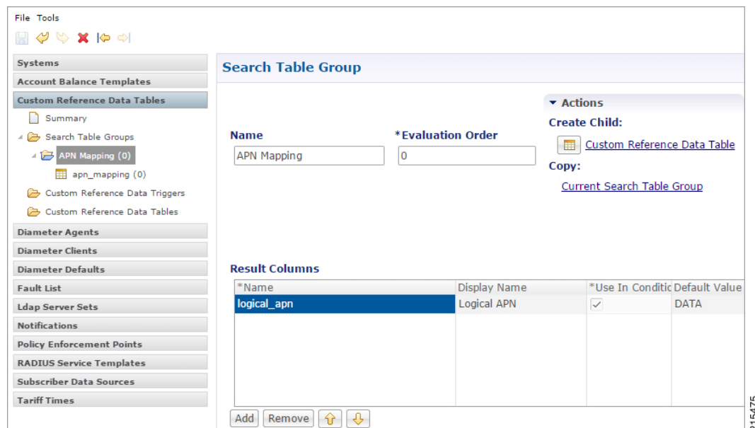
Figure 9: Search Table Group Configuration
