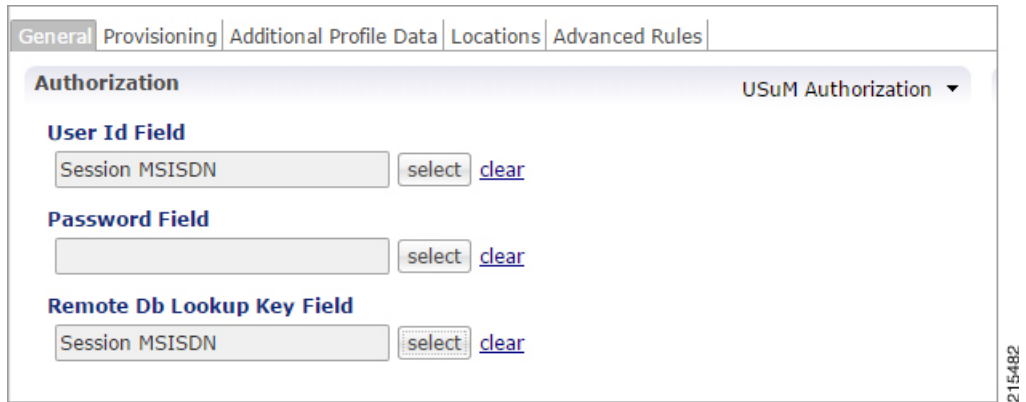
Figure 5: USuM Authorization Configuration
