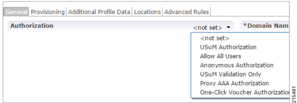
Figure 5: USuM Authorization Configuration
