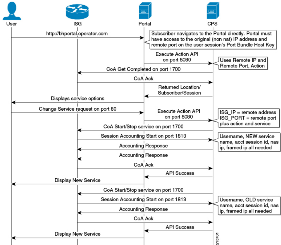
Figure 6: Service Selection Call Flow
