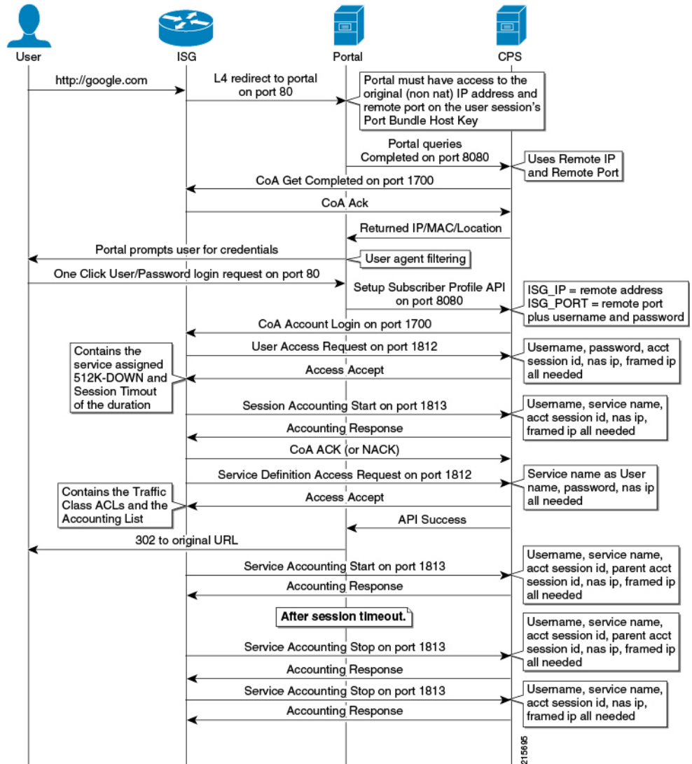
Figure 46: Time-limited Voucher Call Flow
