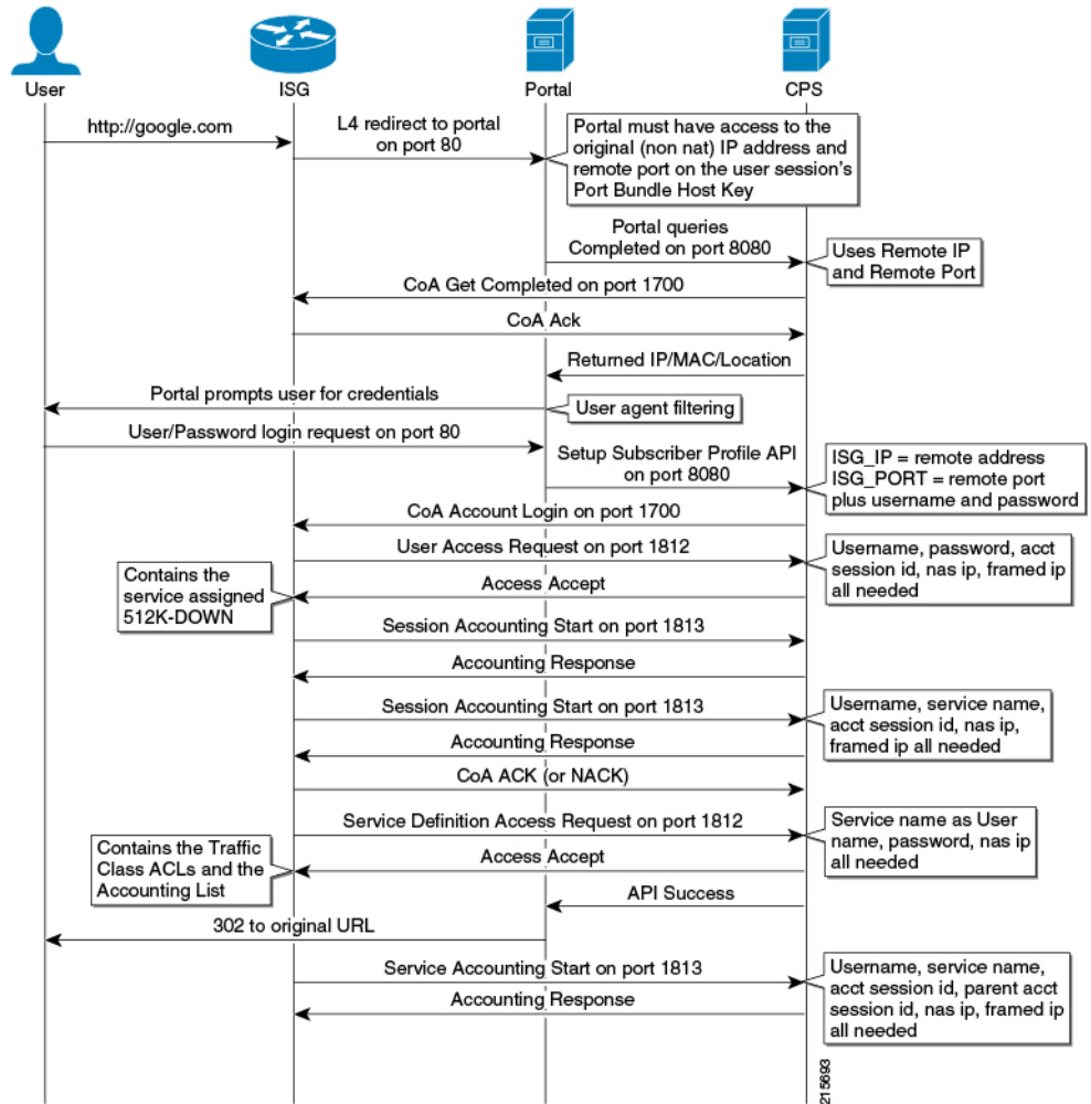
Figure 44: User/Password Login Call Flow
