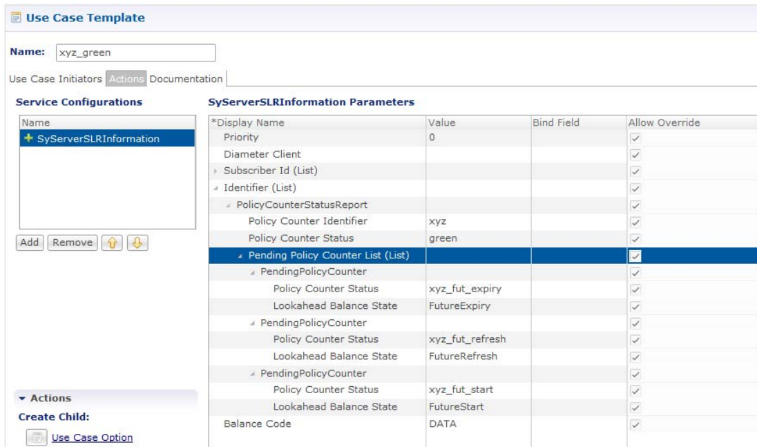
Figure 9: SyServerSLRInformation Service Configuration Object
