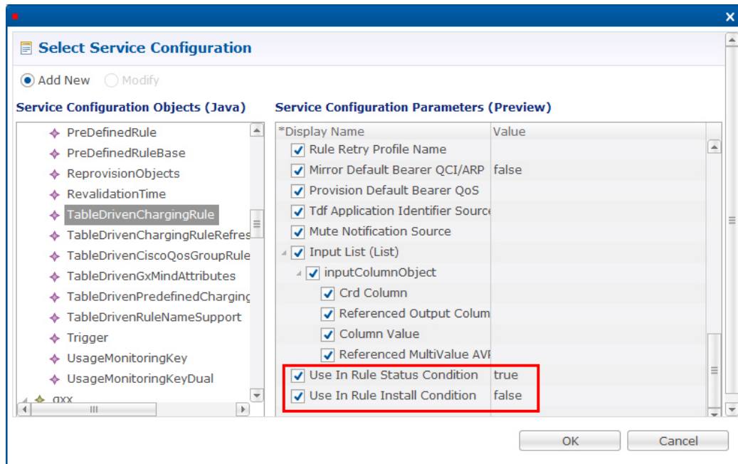
Figure 12: TableDrivenChargingRule
