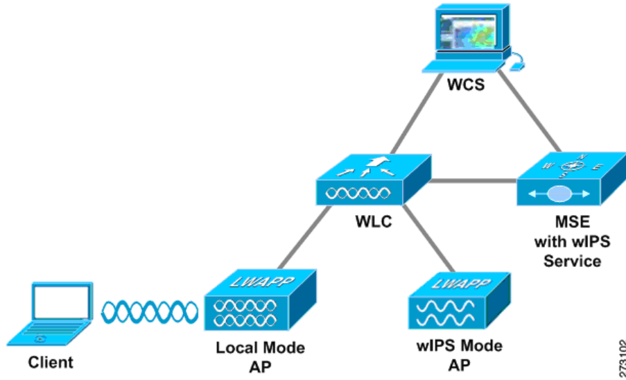
Figure 1-2 wIPS Integrated Within CUWN
