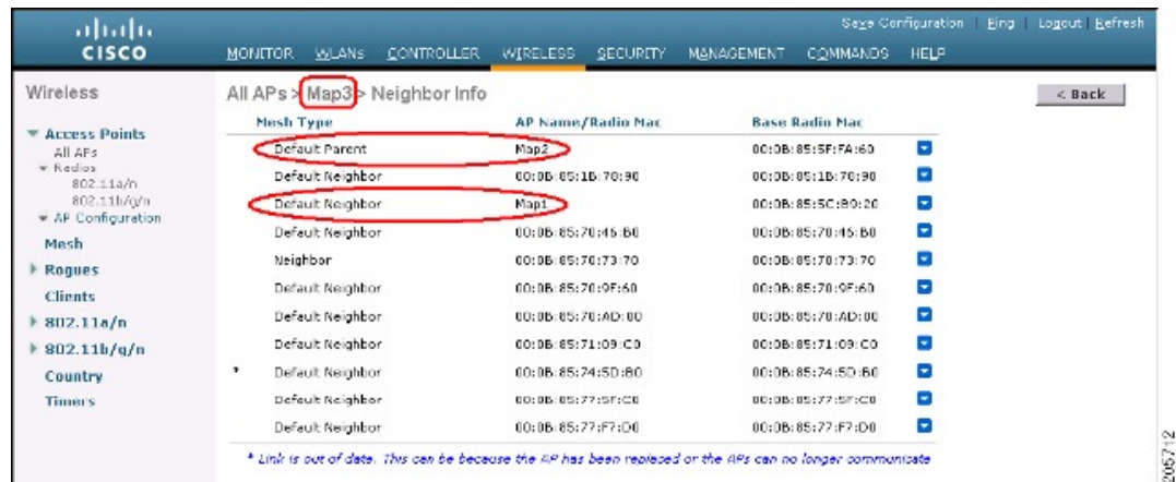
Figure 6: Neighbor Information for a Parent
