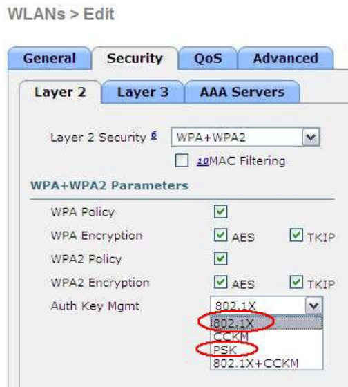
Figure 3: WLAN Security Settings - Auth Key Management
