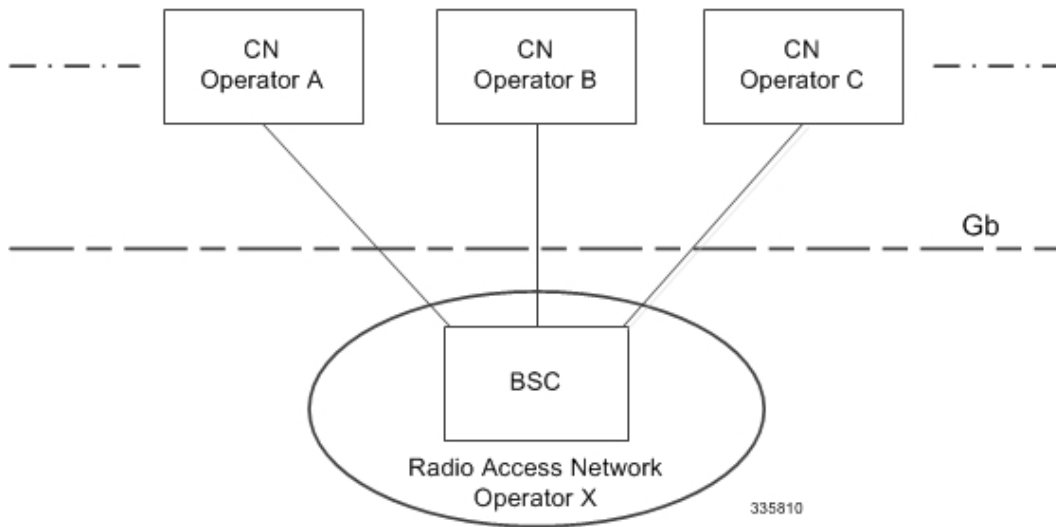
Figure 2: MOCN Configuration
