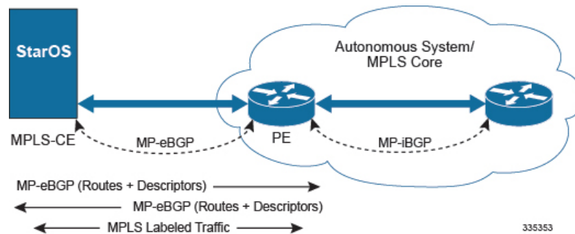
Figure 2: Chassis as MPLS-CE Connected to ASBR
