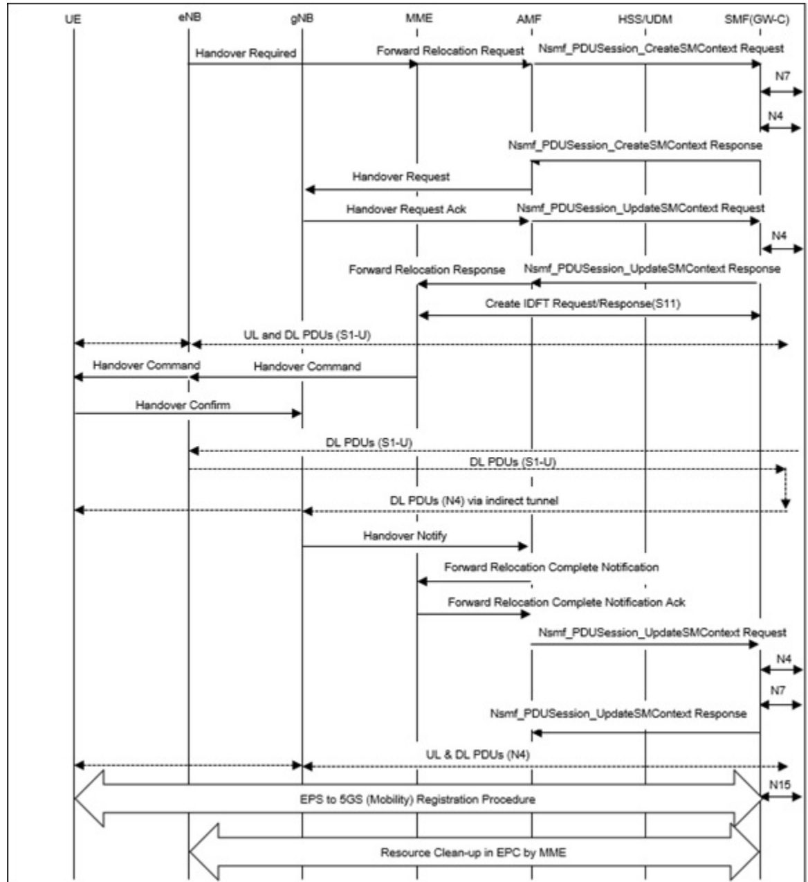
Figure 13: EPS to 5GS Handover
