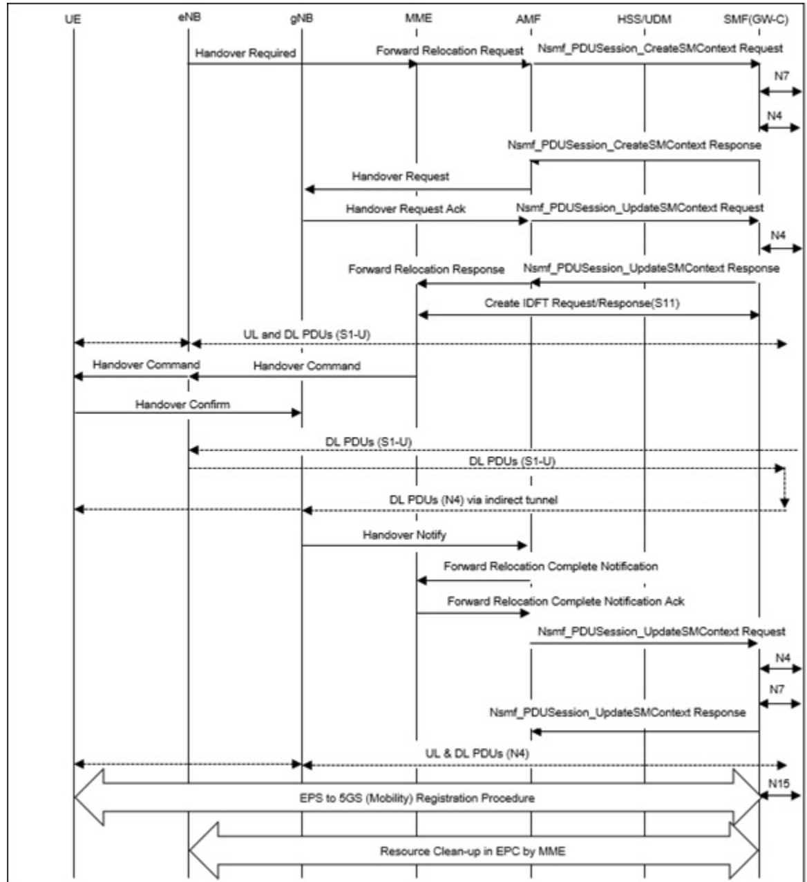
Figure 57: EPS to 5GS Handover
