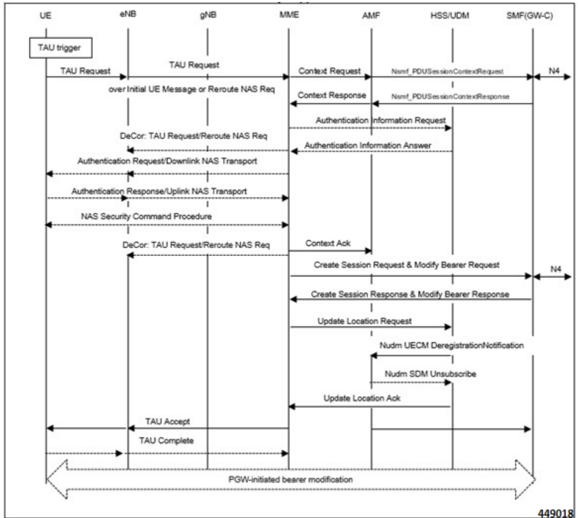
Figure 56: 5GS to EPS Idle Mode Mobility
