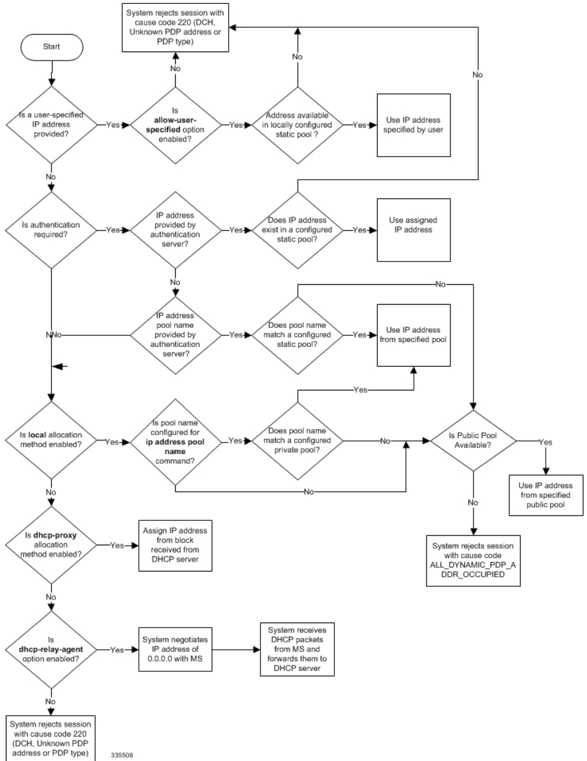
Figure 3: IP Address Allocation Process
