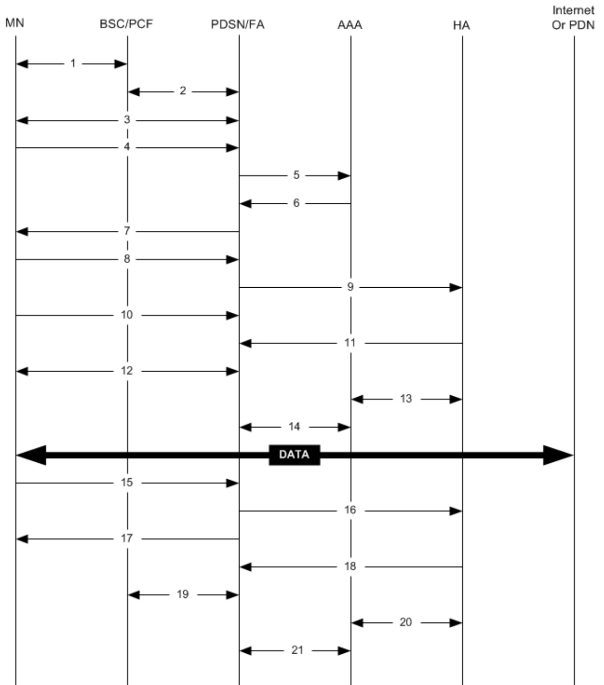
Figure 1: AAA/PDSN Assigned IP Address Proxy Mobile IP Call Flow
